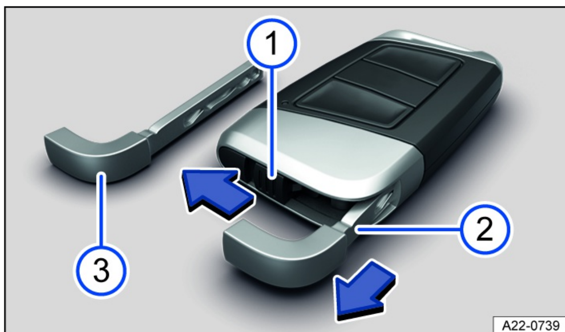
Fig. 53 Vehicle key: Unlocking the emergency key (general example).
