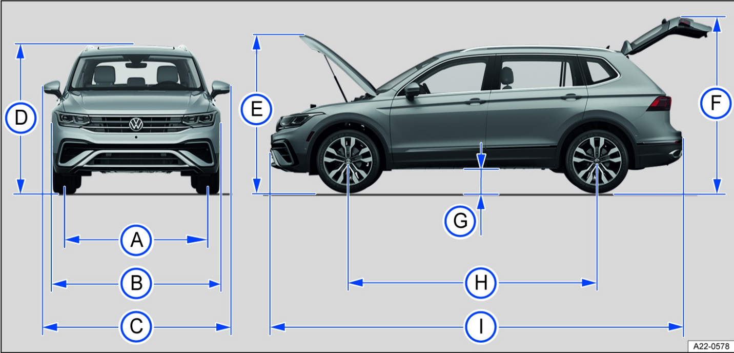
Fig. 239 Vehicle dimensions.
