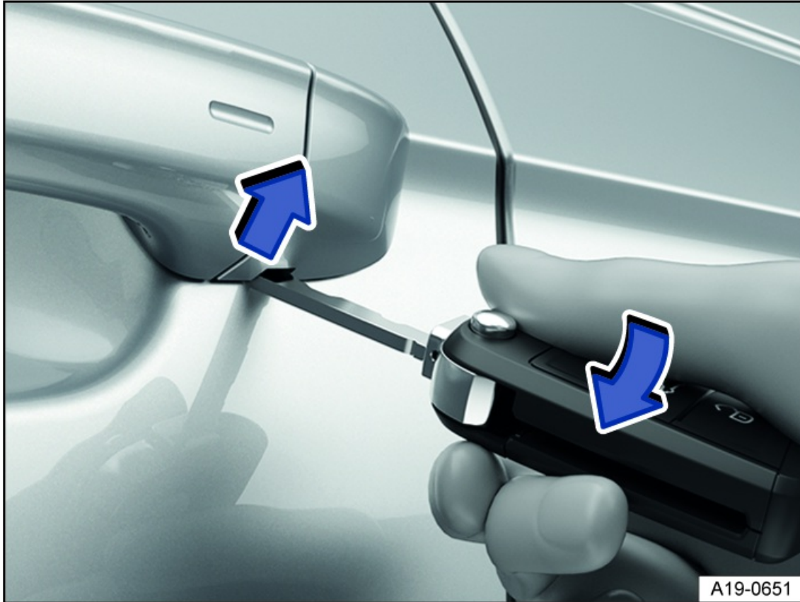
Fig. 61 Driver's door handle: prying off the cap.
