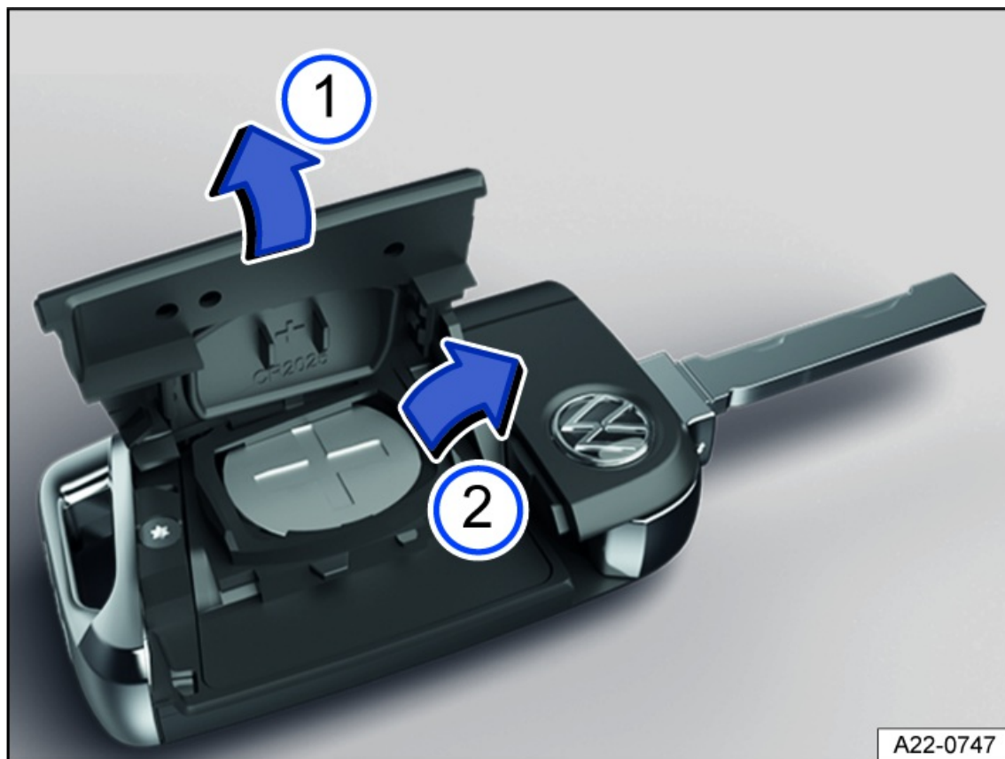
Fig. 54 Vehicle key: Replacing the button cell battery (general example).
