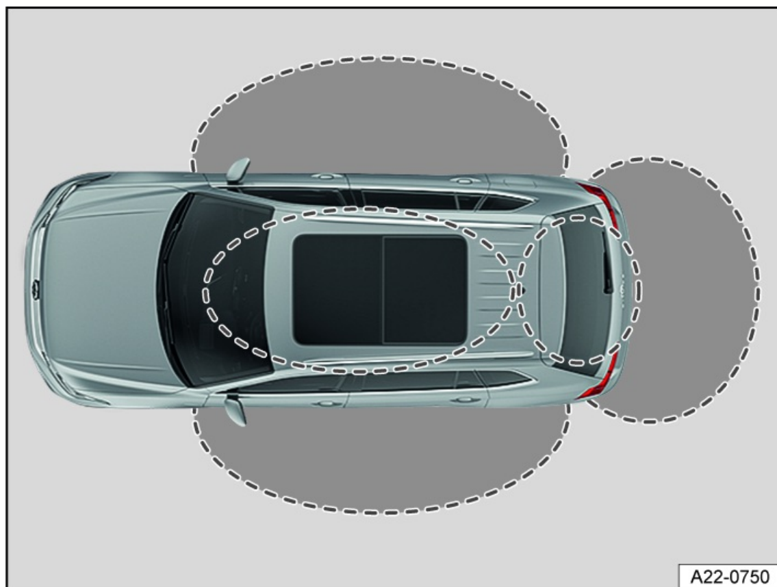
Fig. 57 Keyless Access: Sensor ranges (general example).
