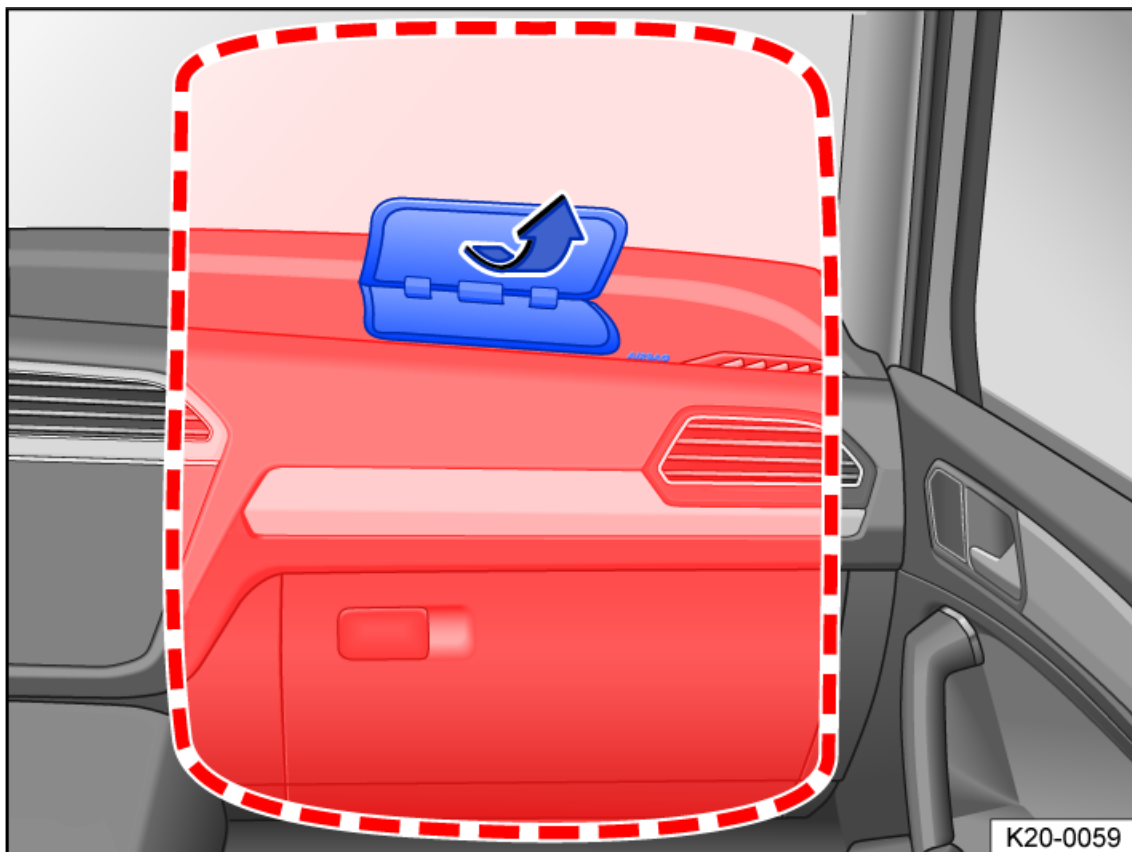
Fig. 37 On the passenger's side: Installation location and deployment zone of the front passenger's front airbag.
