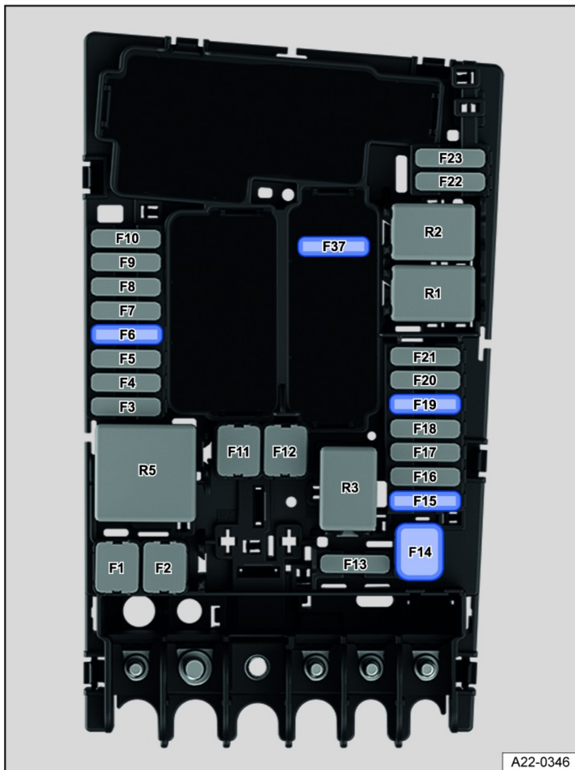
Fig. 192 Fuse locations in the engine compartment.
