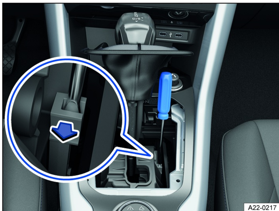
Fig. 125 In the center console: manually release the Automatic Shift Lock (ASL) (variant 2).
