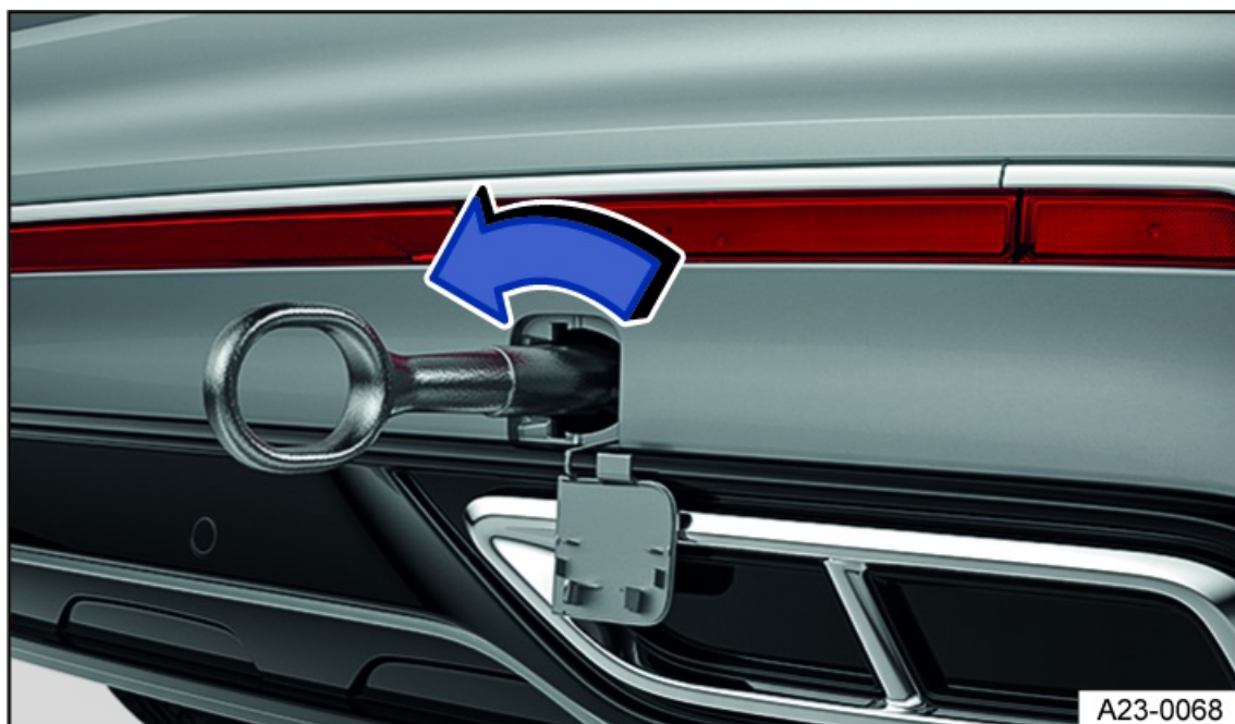
Fig. 205 In the right rear bumper: Screw in towing eye, variant 2.
