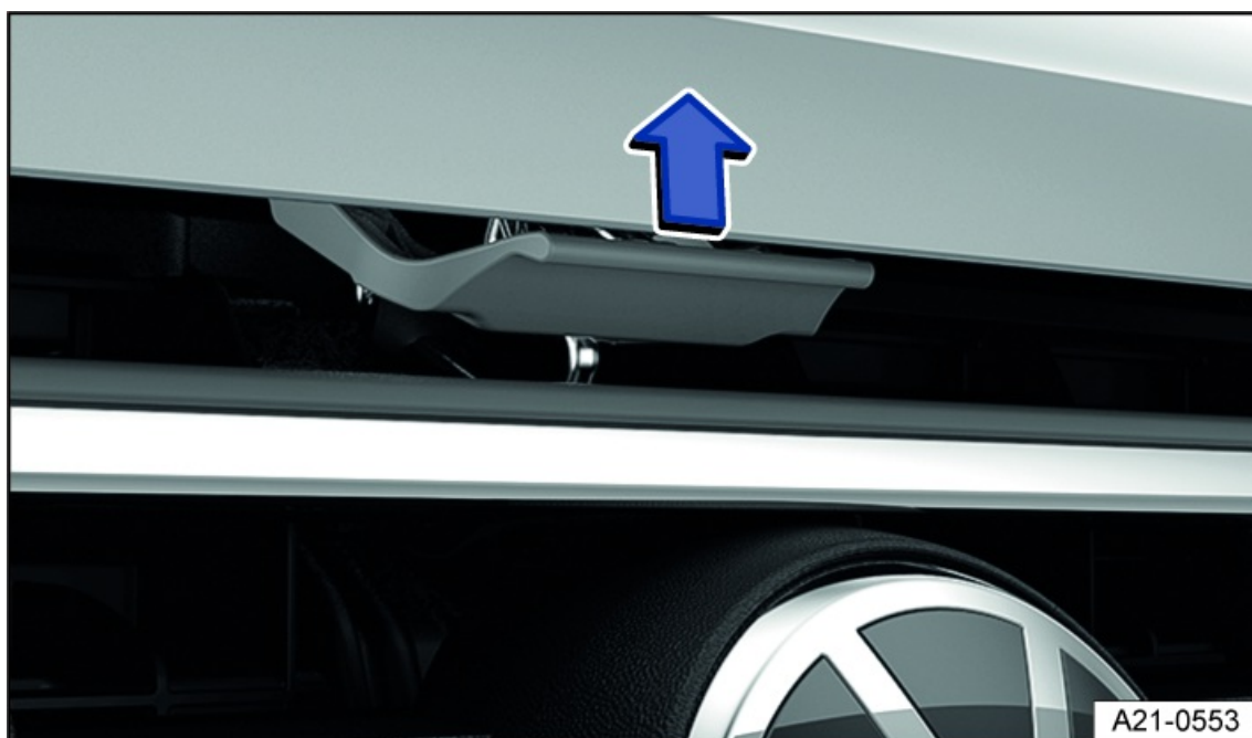
Fig. 207 Above the radiator grille: Opening lever for the hood.
