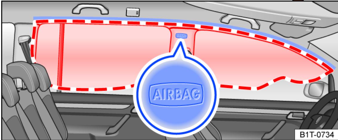
Fig. 40 On the left side of the vehicle (5-seater): installation location and deployment zone of the Side Curtain Protection® airbag.
