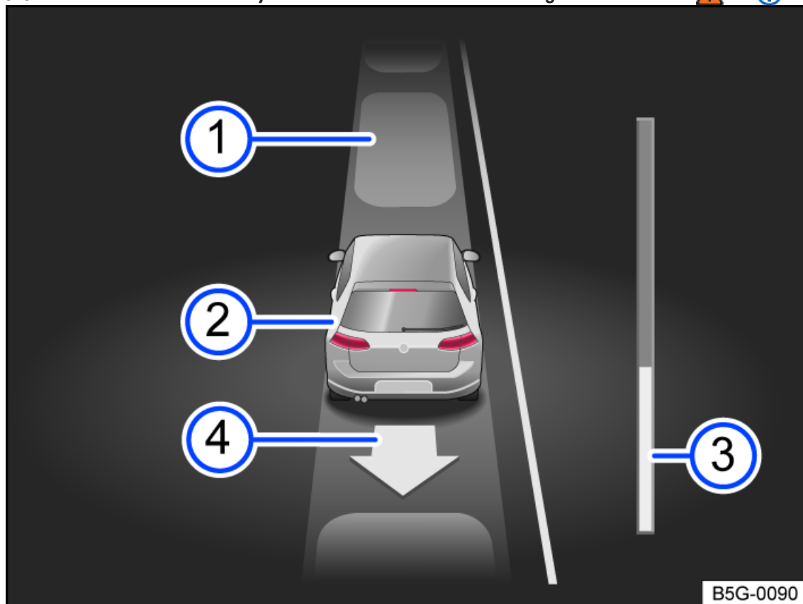
Fig. 159 In the instrument cluster display: reversing out of a parking space parallel to the road.
