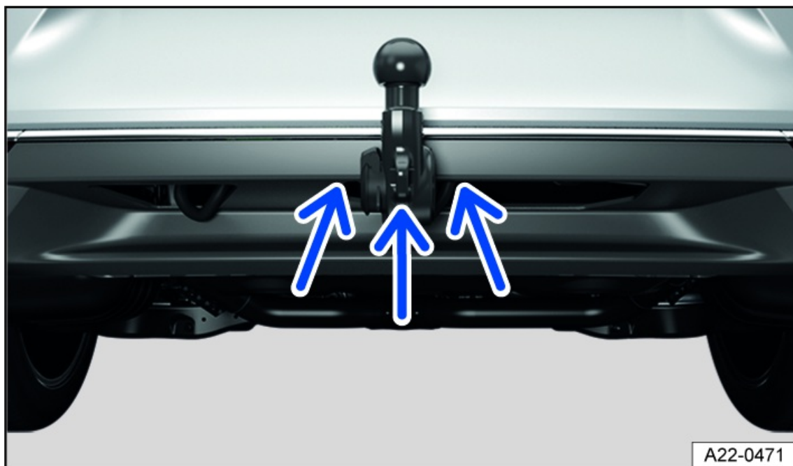
Fig. 181 On the trailer hitch: eye for fastening the securing or breakaway cable (general example).
