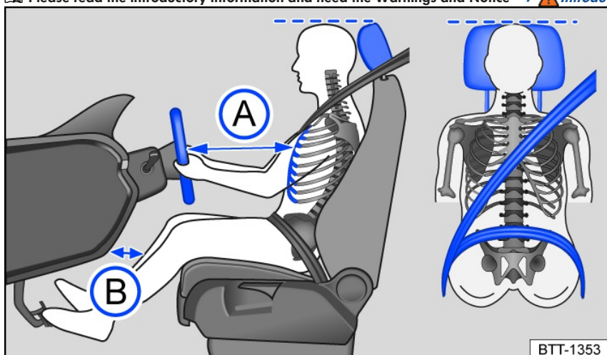
Fig. 19 General example: correct distance between the driver and the steering wheel, correct safety belt routing and correct head restraint adjustment.
