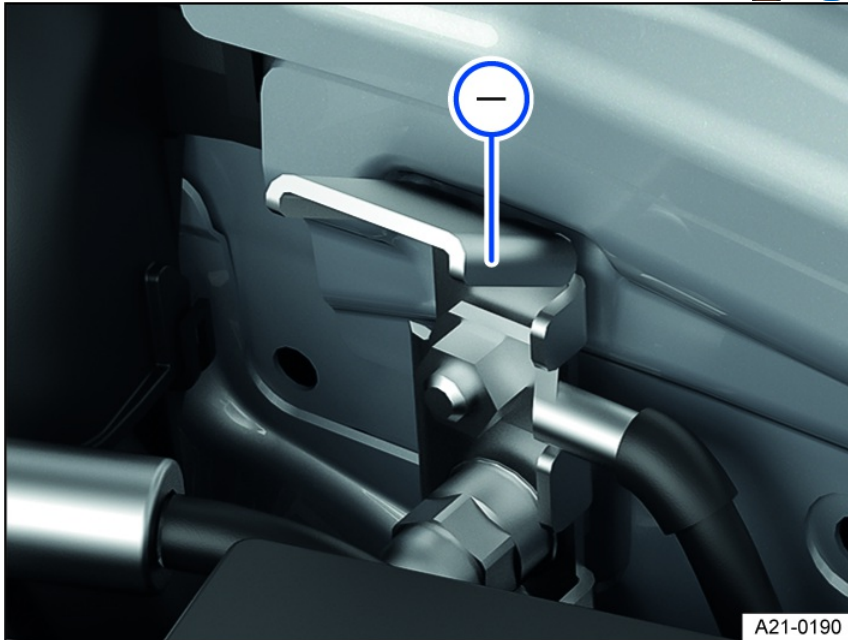
Fig. 142 In the engine compartment: jump-start point (negative terminal).
