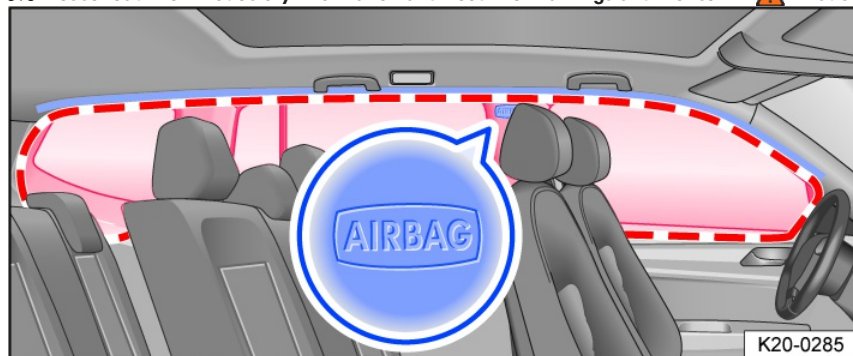
Fig. 31 On the left side of the vehicle: installation location and deployment zone of the Side Curtain Protection®.
