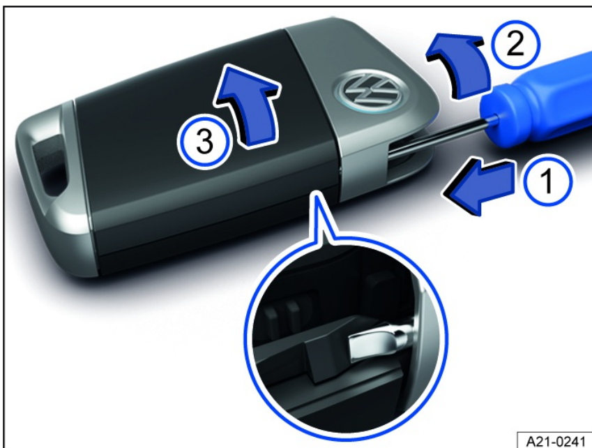
Fig. 44 Vehicle key: opening the battery compartment cover.
