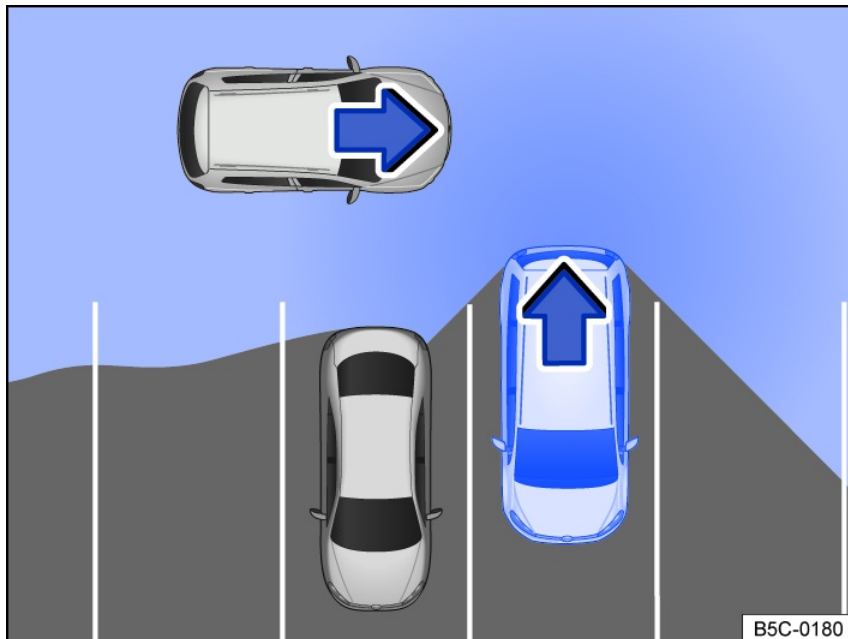
Fig. 118 Rear Traffic Alert, general example: monitored area around the vehicle that is exiting a parking space.
