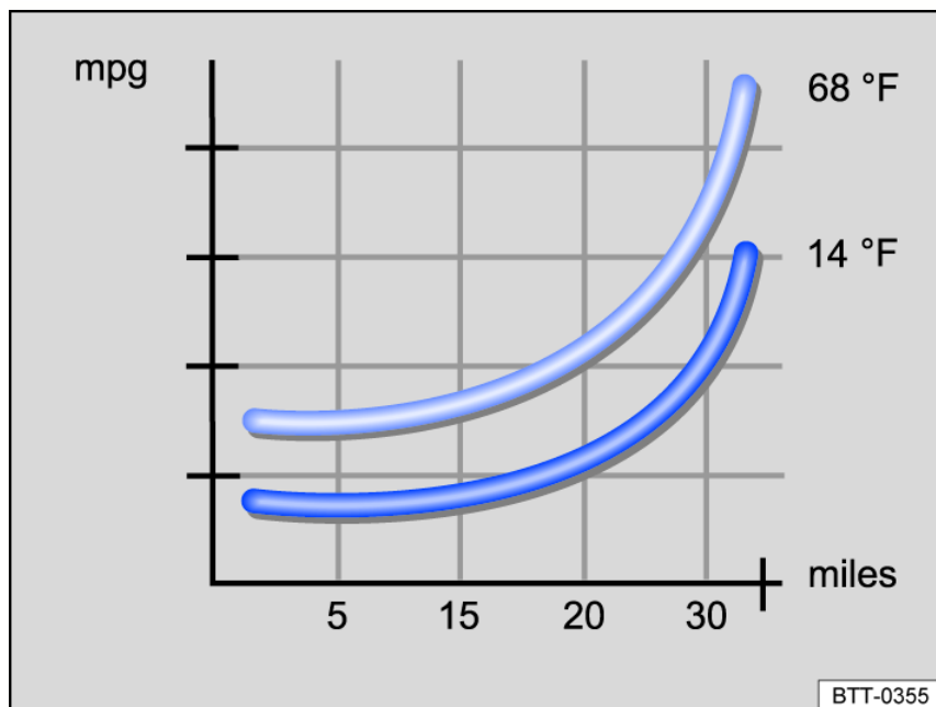
Fig. 86 Fuel consumption in mpg at two different ambient temperatures.
