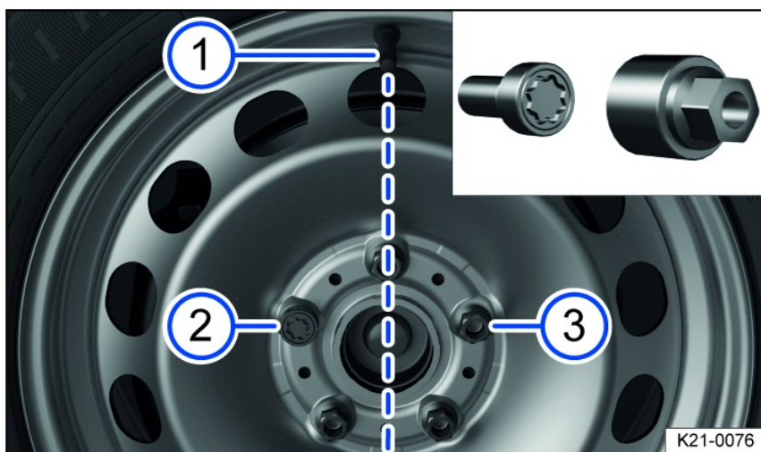
Fig. 169 Changing a tire: tire valve ① and locations of the anti-theft wheel bolt ② or ③.
