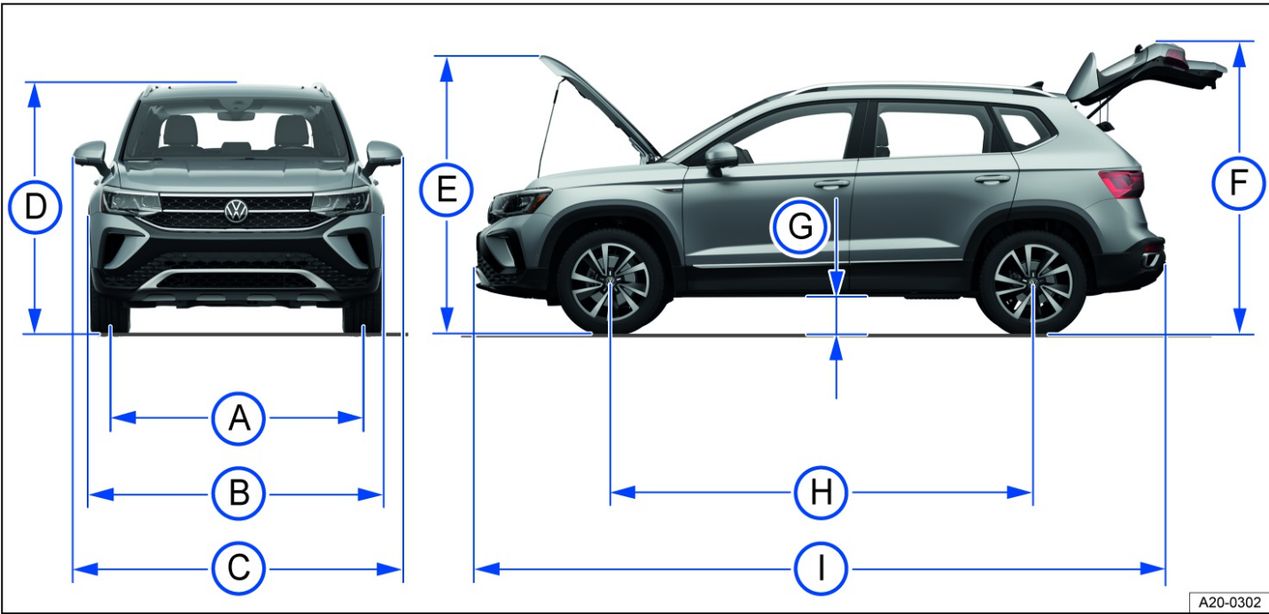
Fig. 184 Vehicle dimensions.
