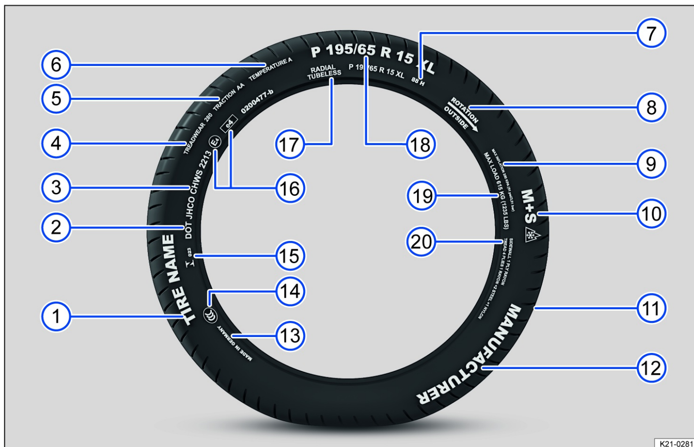
Fig. 164 International tire labeling.
