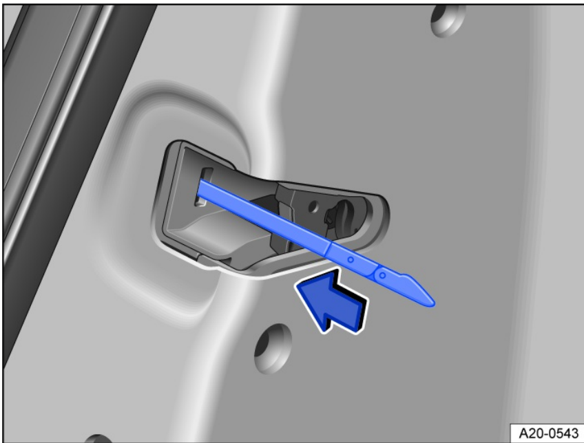
Fig. 51 In the front edge of the rear right-hand door: Vehicle emergency lock for using the emergency key (variant 2).
