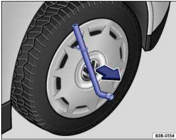
Fig. 161 Pulling the wheel cover off.
