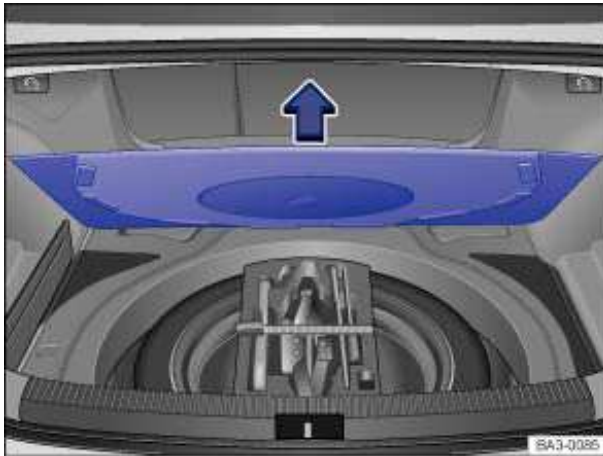
Fig. 157 In the luggage compartment under the floor panel: Compact spare wheel and vehicle tool kit.
