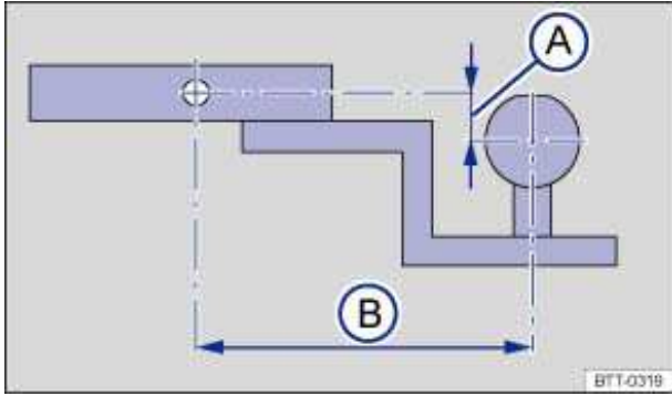
Fig. 87 Dimensions of the ball mount support.
