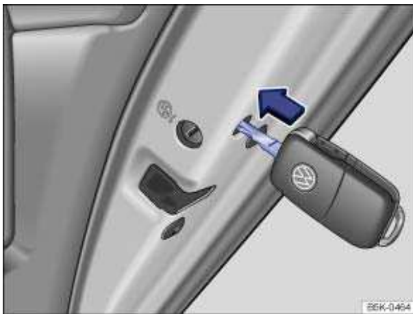
Fig. 150 On the front side of the right rear door: Manual vehicle locking with the key bit in the vehicle key.
