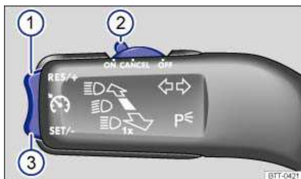
Fig. 121 On the left side of the steering column: Cruise control buttons and switches.
