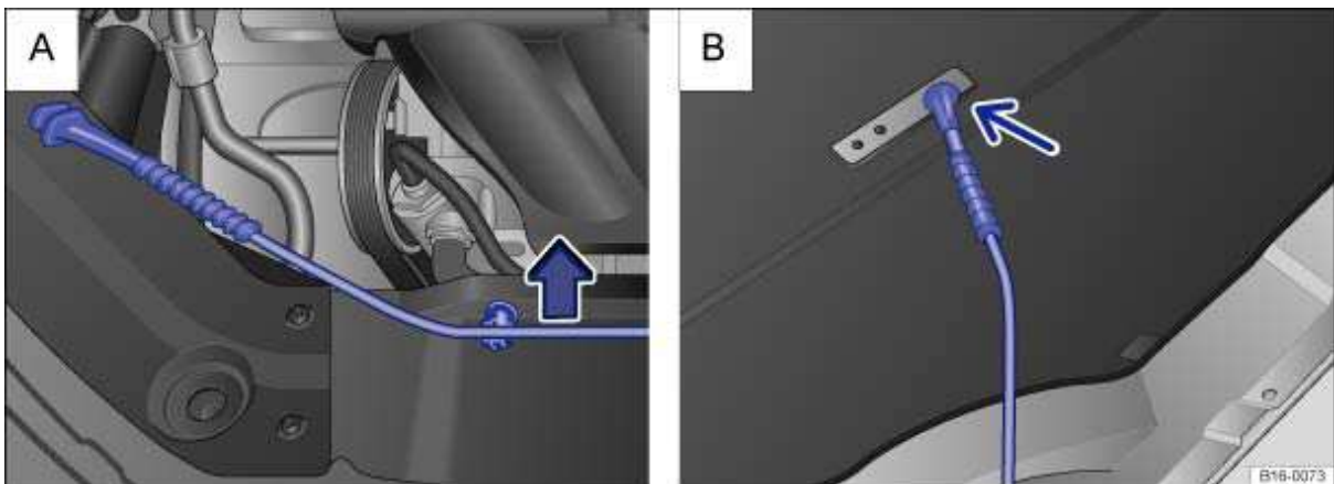
Fig. 131 A: In the engine compartment: Bracket for hood support. B: Hood propped open.
