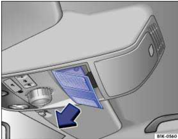
Fig. 153 In headliner: Removing cover.
