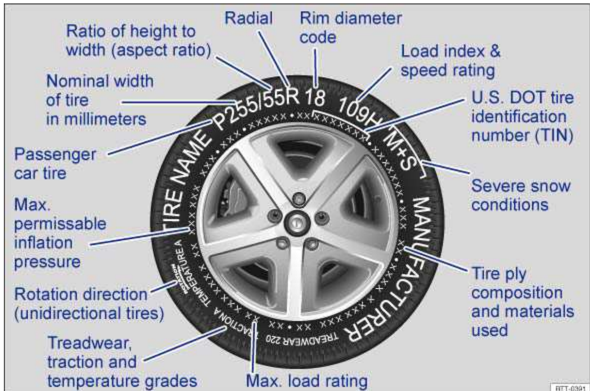
Fig. 144 International tire labeling.
