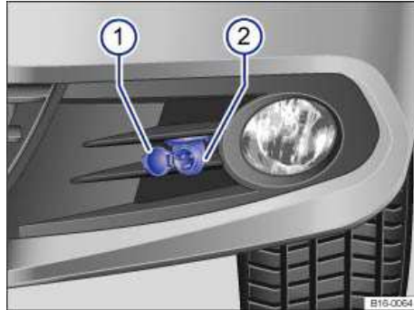
Fig. 106 In the front left bumper: Connection socket 2 for the engine preheating system.
