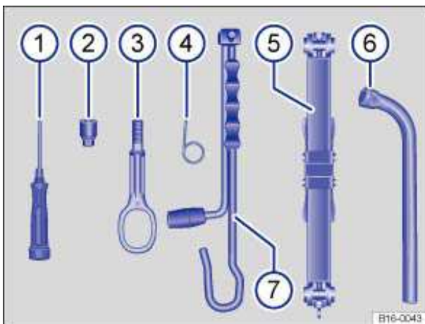
Fig. 158 Contents of the vehicle tool kit.
