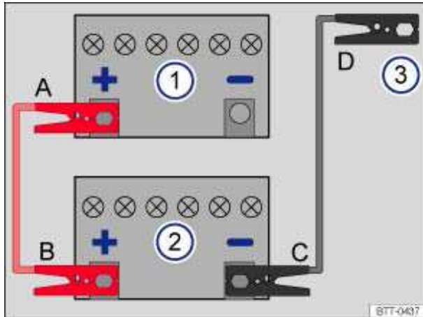
Fig. 181 Diagram for attaching the jumper cables: Dead battery 1 and booster battery 2.
