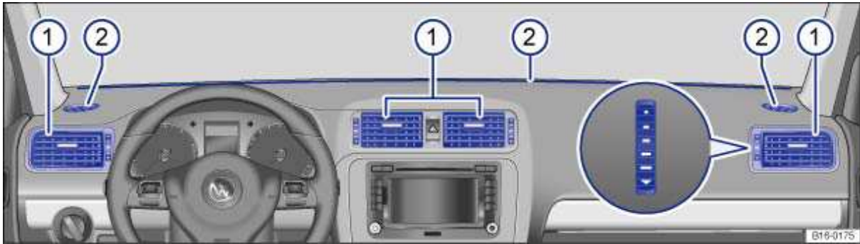
Fig. 125 In the instrument panel: Air vents.
