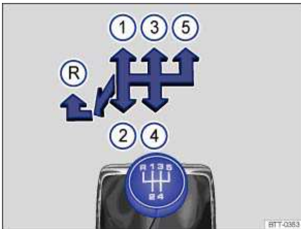
Fig. 109 Gearshift pattern of a 5-speed manual transmission.
