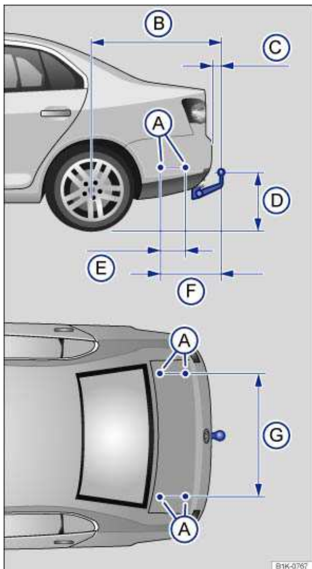
Fig. 88 Dimensions and attachment points for retrofitting a trailer hitch.
