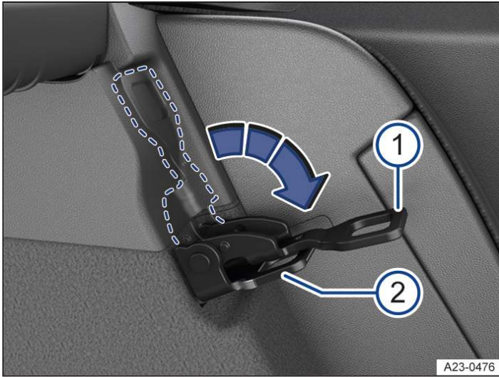
Fig. 1 In the luggage compartment: bracket for backrest angle.
