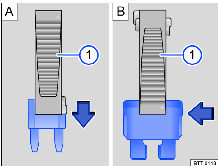
Fig. 2 Removing or inserting fuse with plastic pliers (illustration).
