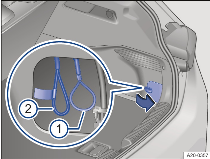
Fig. 1 Behind a flap in the right-hand luggage compartment trim: Manual release mechanism for the charging connector (1) and emergency cut-out connection (2).
