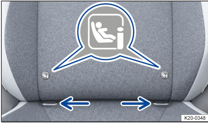
Fig. 3 Markings identifying the i-Size anchorage points for child seats on the front passenger seat.
