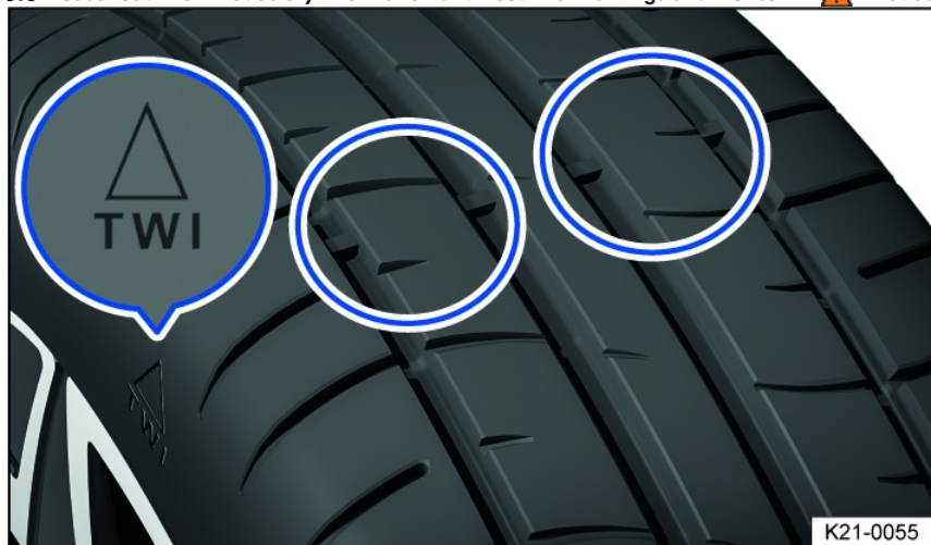
Fig. 196 Tire tread: tread wear indicator.
