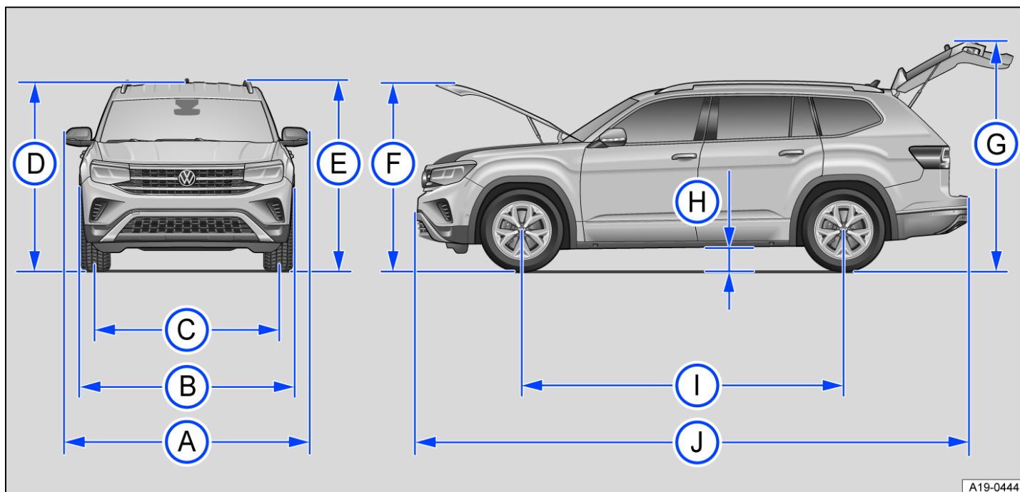
Fig. 215 Vehicle dimensions.
