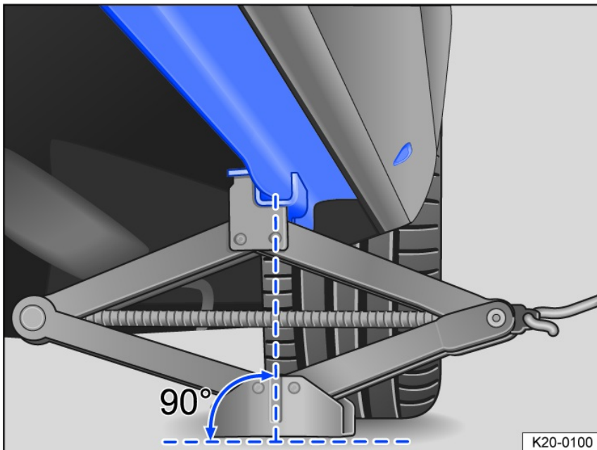
Fig. 206 Jack is positioned on the left side of the vehicle at the rear.
