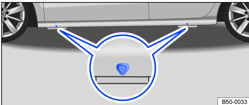
Fig. 204 Lift points for the vehicle jack (general example).
