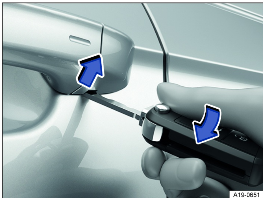
Fig. 55 Driver's door handle: prying off the cap.
