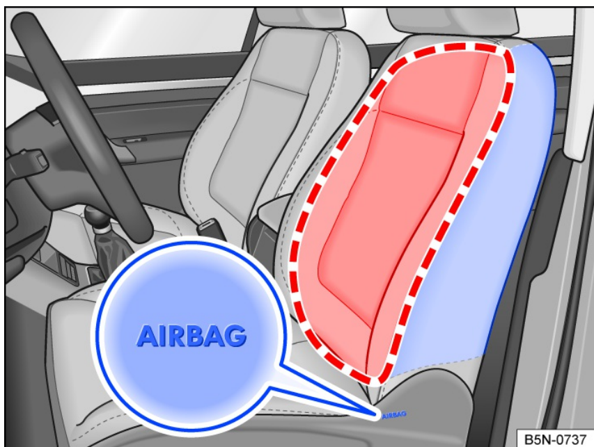
Fig. 31 On the side of the front seat: Side airbag installation location and deployment zone
