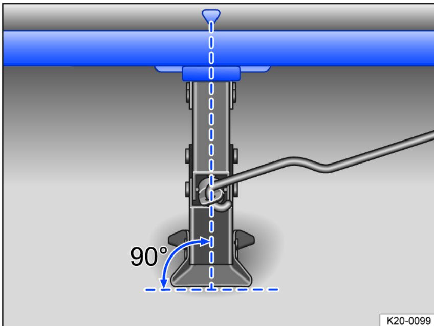
Fig. 205 Correct jack setup.
