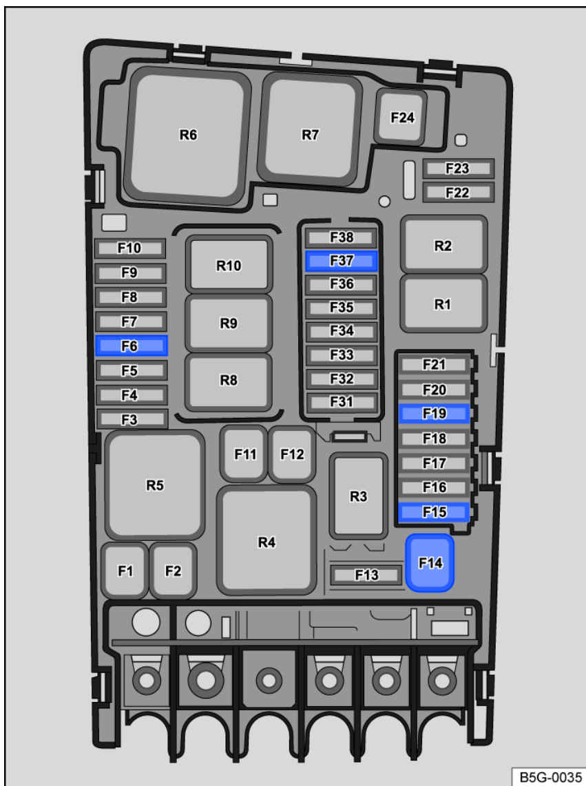
Fig. 174 Fuse locations in the engine compartment.
