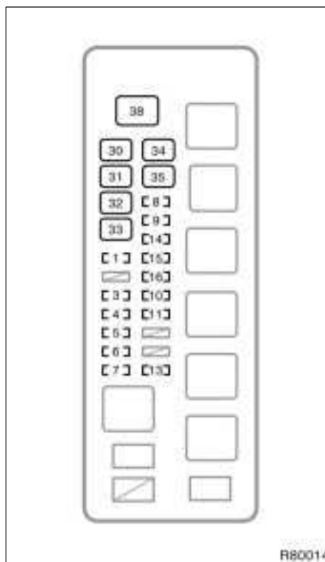
Engine compartment (5VZ-FE engine)
