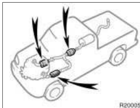
2UZ-FE engine (type B)
