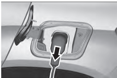
275 Disconnect the vehicle plug of the charging cable from the charging port fig. 275 within 30 seconds after unlocking. JJ000473
