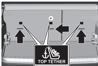
157 JJ000796 (*) Depending on country of sale In addition to the ISOFIX brackets, fasten the Top-tether strap to the Top-tether anchors.
