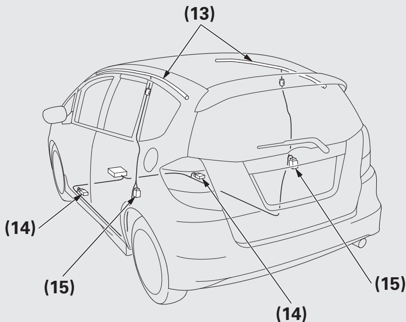
(13) Side Curtain Airbags (14) Side Impact Sensors (First) (15) Side Impact Sensors (Second)
