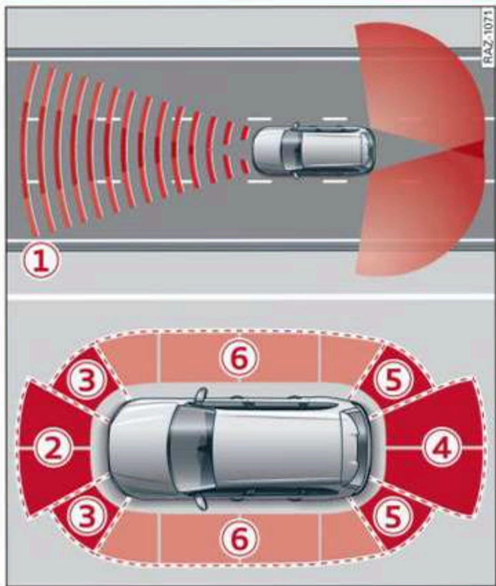
Fig. 96 Sensor detection ranges
