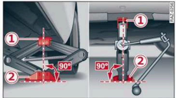
Fig. 173 Sill: positioning the vehicle jack
