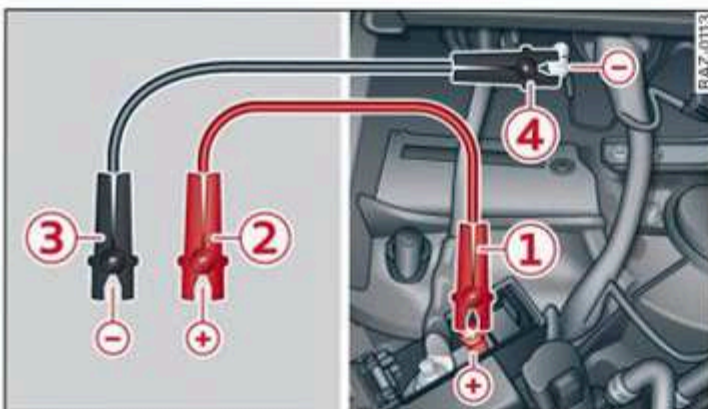
Fig. 177 Connecting the jump start cables
