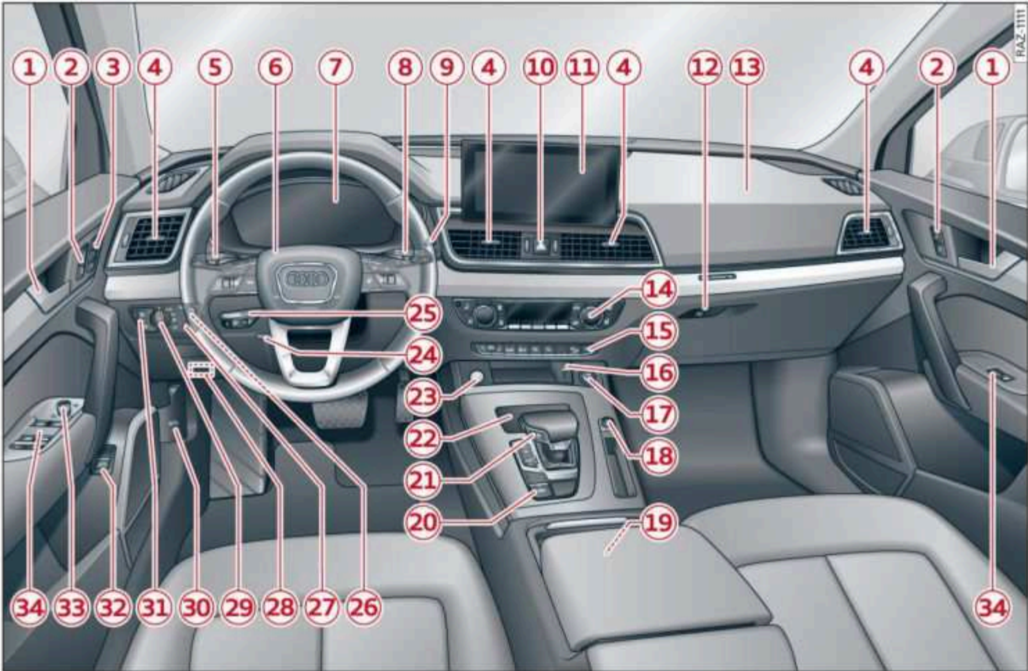
Fig. 1 Cockpit
