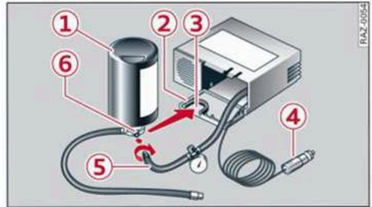
Fig. 168 Components of the tire mobility kit
