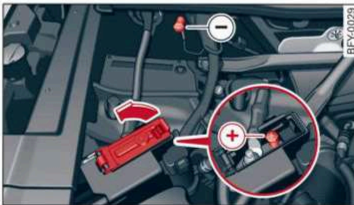
Fig. 176 Engine compartment: connectors for jump start cables or a charger
