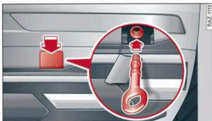
Fig. 179 Rear bumper: installing the towing loop (version 1)
