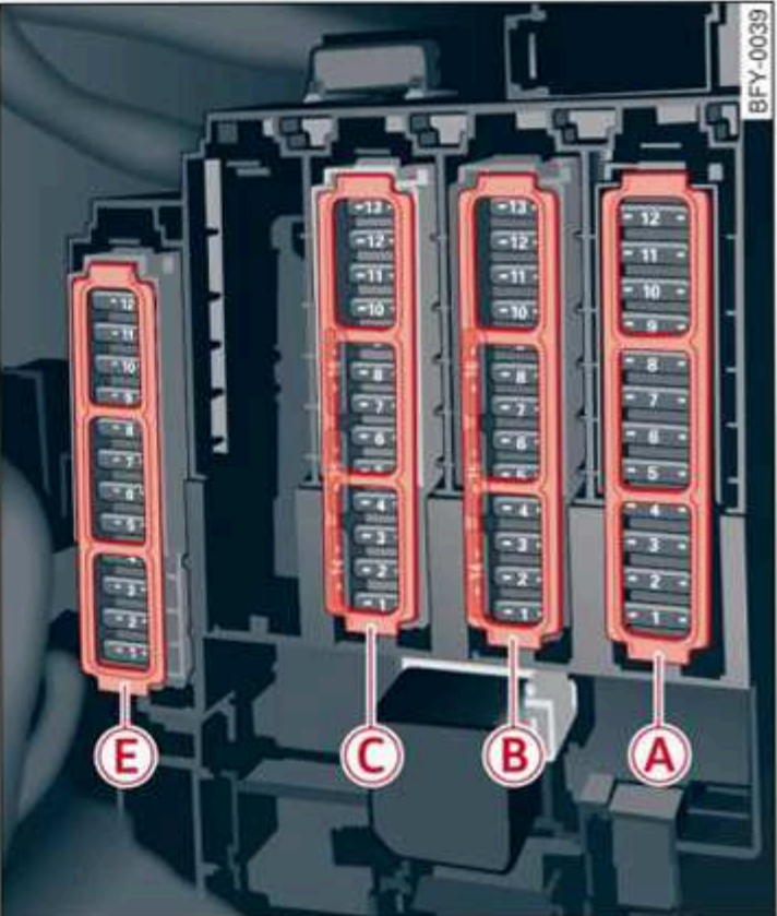
Fig. 186 Left side of the luggage compartment: fuse panel with plastic clip
