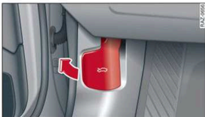
Fig. 153 Footwell: release lever
