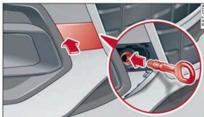
Fig. 178 Front bumper: installing the towing loop
