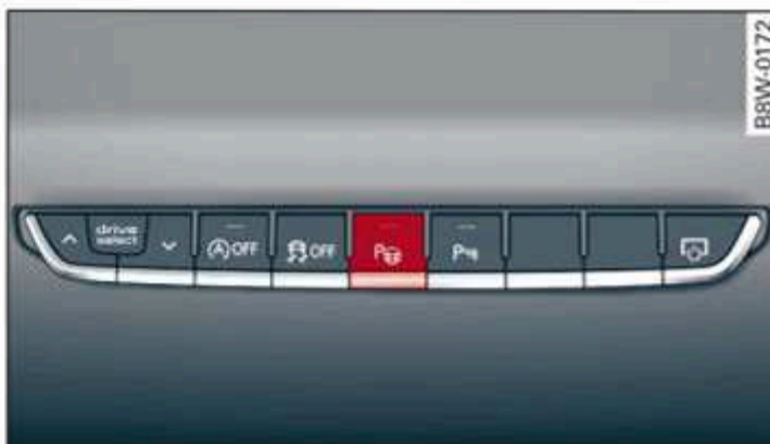
Fig. 130 Center console: park assist button
