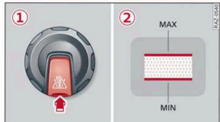
Fig. 158 Engine compartment - Coolant expansion tank (diagram): ① cover with release button; ② markings
