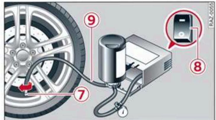
Fig. 169 Tire mobility kit connection
