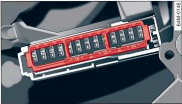
Fig. 185 Driver side cockpit: fuse panel with plastic bracket
