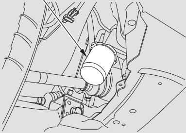
OIL FILTER
