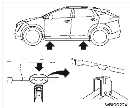
jack-up points
