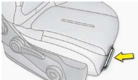
Forwards-backwards
