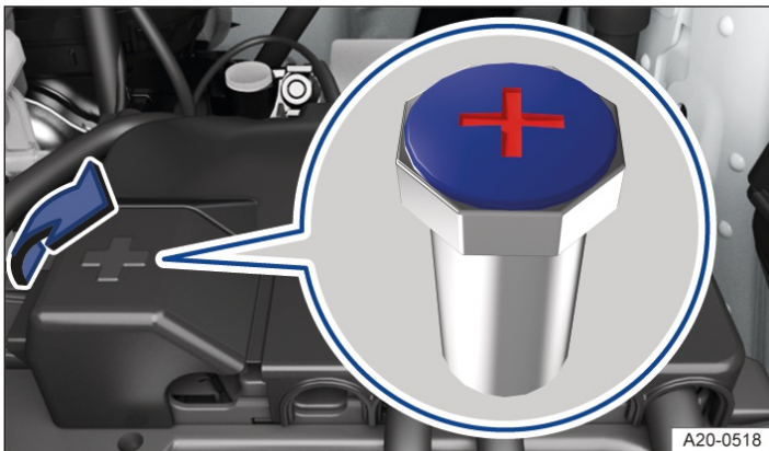
Fig. 1 In the bonnet space underneath a cover: jump-start connection point (positive battery terminal).
