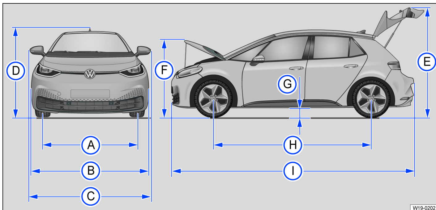
Fig. 1 Dimensions.
