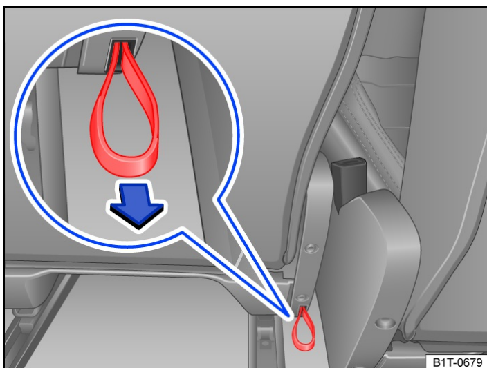
Fig. 2 Second row of seats: loop for the emergency exit function for the third row of seats.
