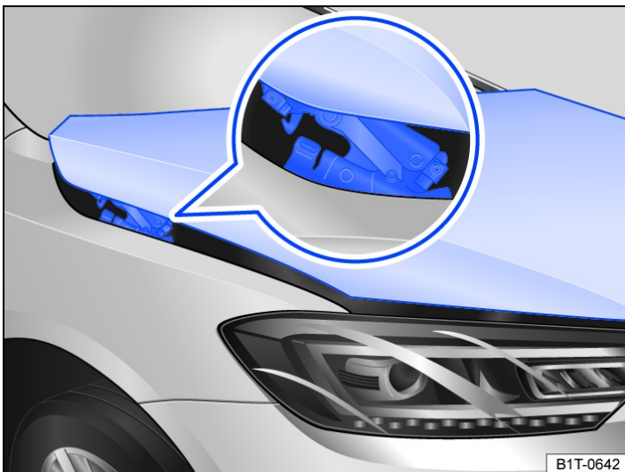
Fig. 1 Triggered re-active bonnet (illustration).
