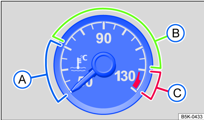
Fig. 1 Coolant temperature display in the analogue instrument cluster (schematic diagram).
