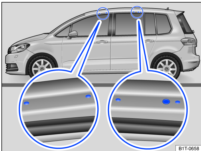
Fig. 1 Mounting points for base carriers (vehicles without roof rails).
