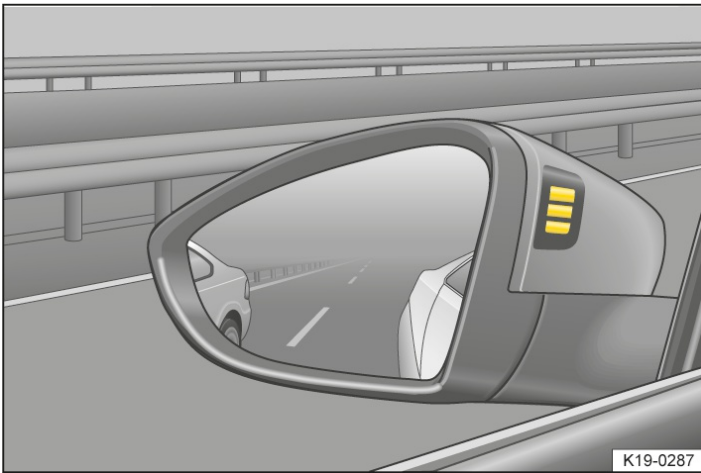
Fig. 1 In the wing mirror housing: visual displays for the lane change system.
