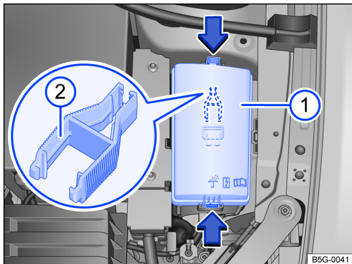
Fig. 1 In the engine compartment: cover (1) of the fuse box including plastic pliers (2).
