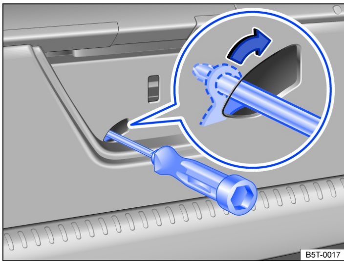
Fig. 2 In the boot lid: manual release mechanism for the boot lid.
