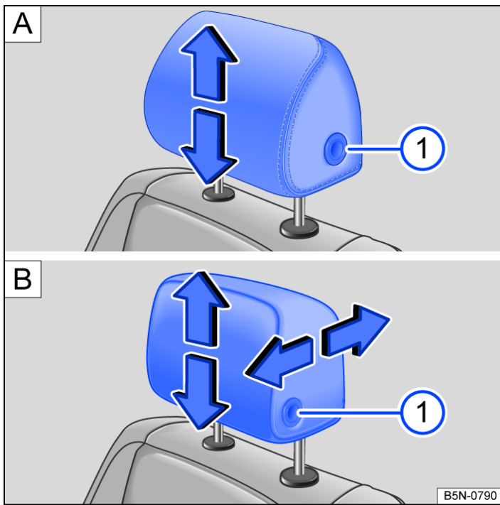
Fig. 1 Adjusting the front head restraints: A without longitudinal adjustment, B with longitudinal adjustment.
