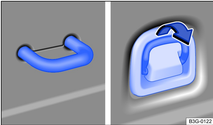
Fig. 1 In the luggage compartment: fixed and folding fastening rings.
