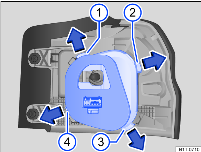
Fig. 2 Tail light cluster in the body: removing the bulb holder.
