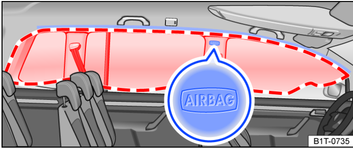
Fig. 2 On the left-hand side of the vehicle(7-seater): location and deployment zone of the curtain airbag.
