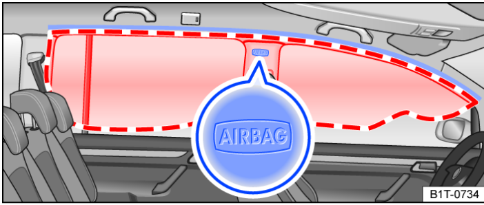
Fig. 1 On the left-hand side of the vehicle(5-seater): location and deployment zone of the curtain airbag.
