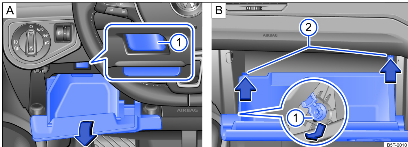
Fig. 1 Fuse box cover in the dash panel: A : left-hand drive vehicle, to the left-hand side of the steering wheel B : Right-hand drive vehicle, on the front passenger side.
