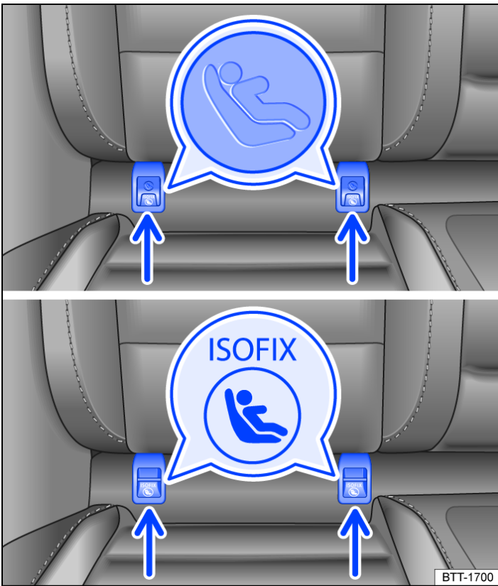
Fig. 1 Markings identifying the ISOFIX anchor points for child seats.
