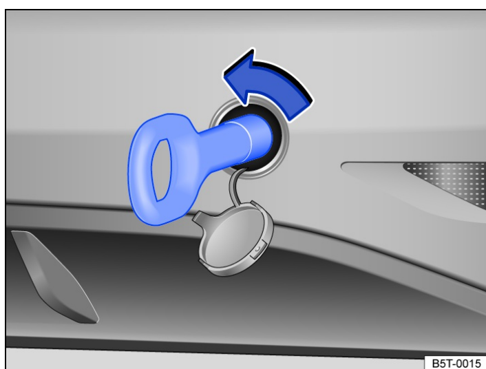
Fig. 2 In the rear bumper on the right: screwing in the towing eye.
