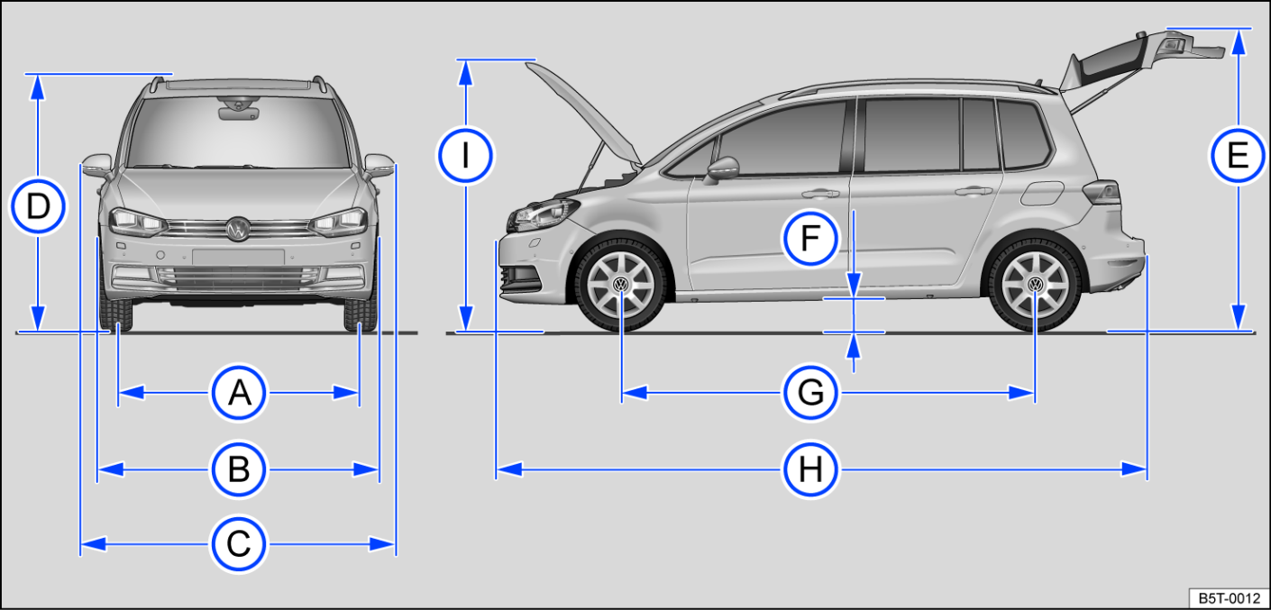
Fig. 1 Dimensions.
