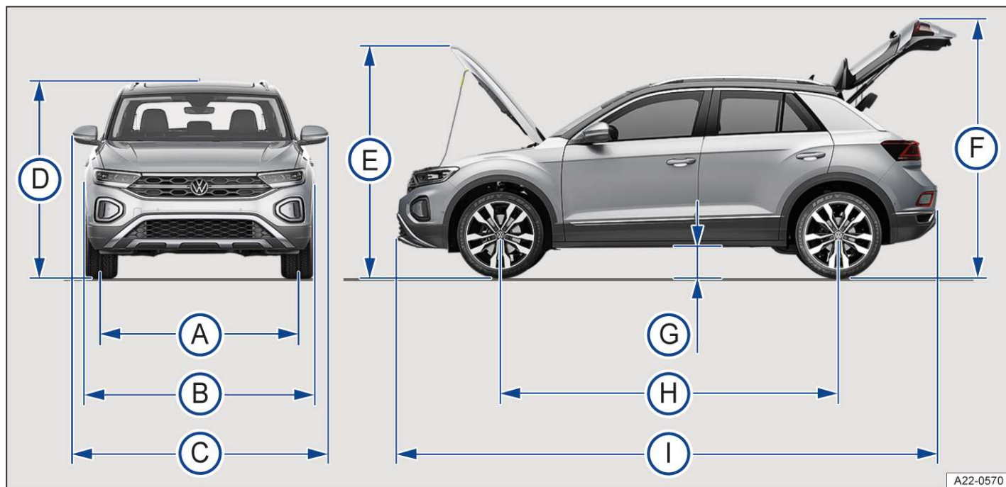
Fig. 1 Vehicle dimensions.
