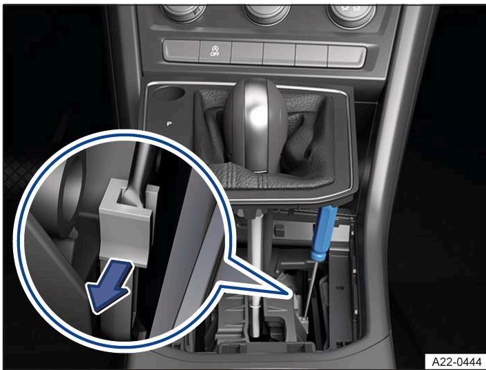
Fig. 2 In the centre console: releasing the selector lever lock manually (variant 2).
