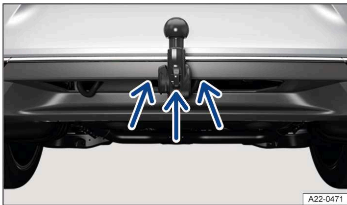
Fig. 1 On the towing bracket: eye for securing the safety or breakaway cable (illustration).
