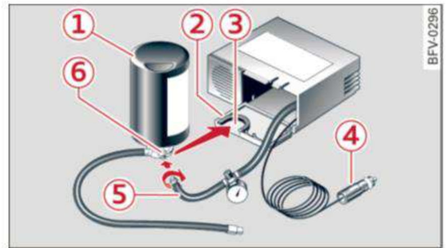
Fig. 272 Components of the tire mobility kit
