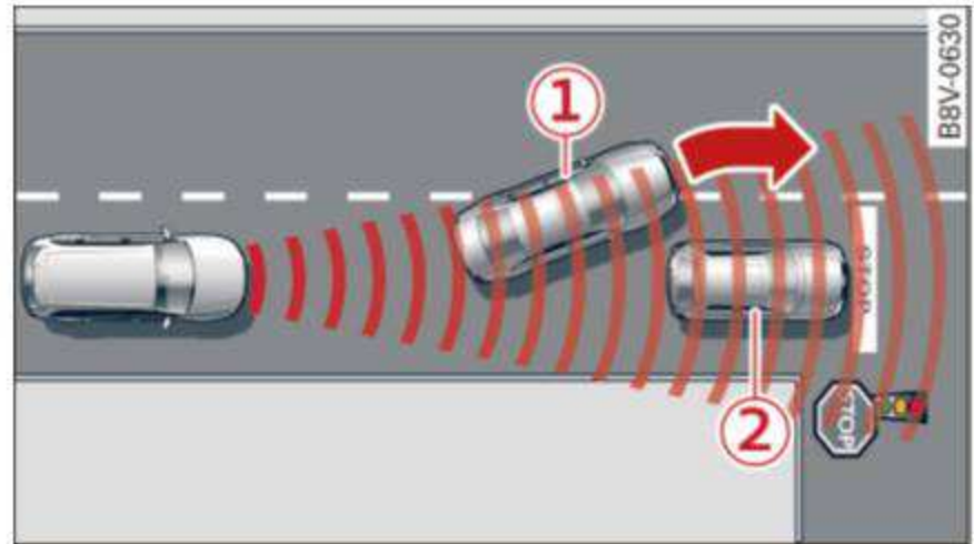
Fig. 102 Example: vehicle changing lanes and stationary vehicle
