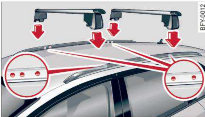
Fig. 80 Roof: mounting points for the roof rack
