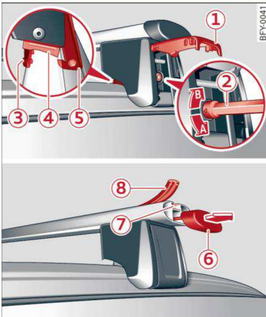
Fig. 81 Roof rail: installing a roof rack
