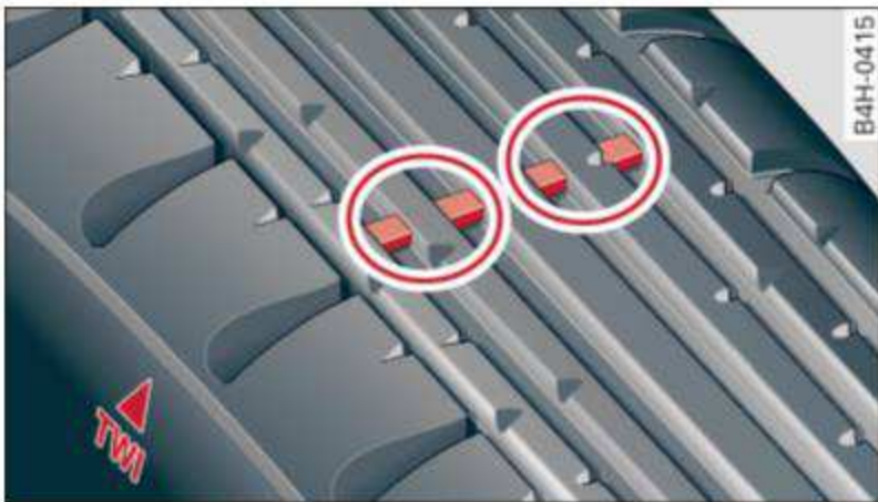
Fig. 267 Tire profile: treadwear indicator
