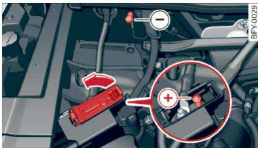
Fig. 286 Engine compartment: connectors for jump start cables and a charger
