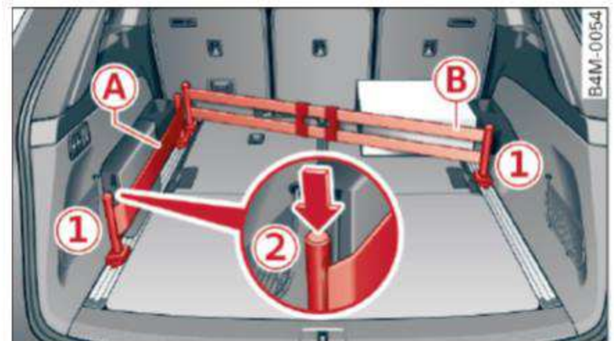
Fig. 76 Luggage compartment: securing attachments
