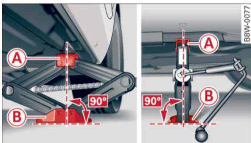
Fig. 277 Sill: positioning the vehicle jack
