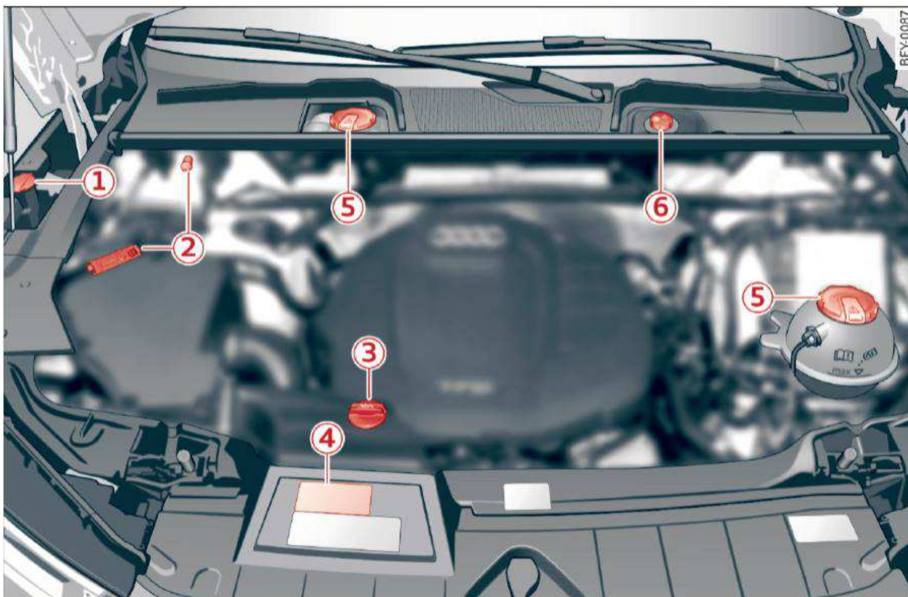
Fig. 260 Typical location of the reservoir and the engine oil filler opening
