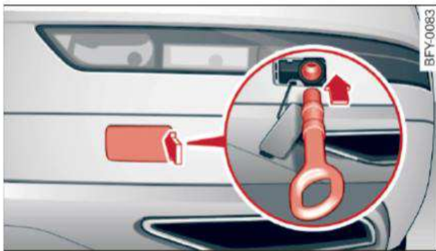
Fig. 289 Rear bumper: installing the towing loop
