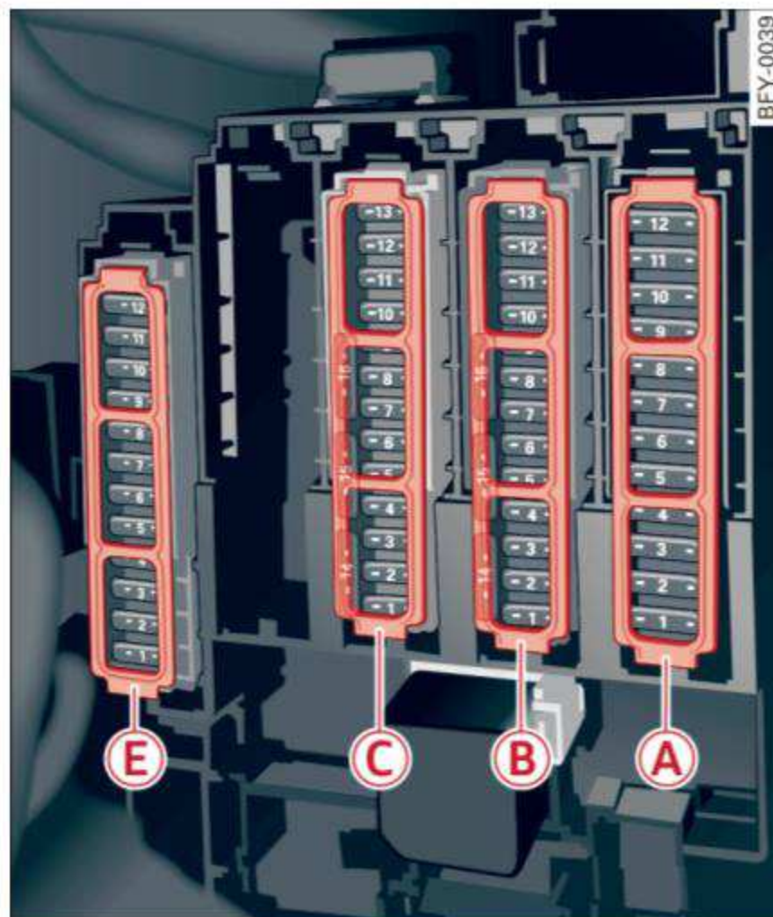
Fig. 285 Left side of the luggage compartment: fuse panel with plastic clip
