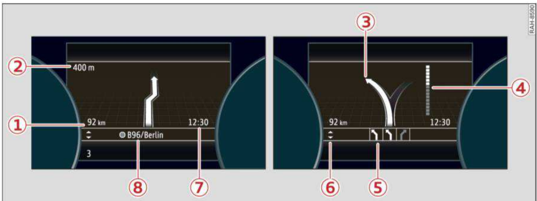
Fig. 170 Example: arrow view (monochrome instrument cluster)
