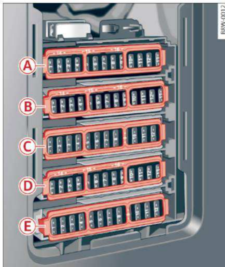
Fig. 283 Front passenger's footwell (right-hand drive vehicle): fuse panel with plastic clip
