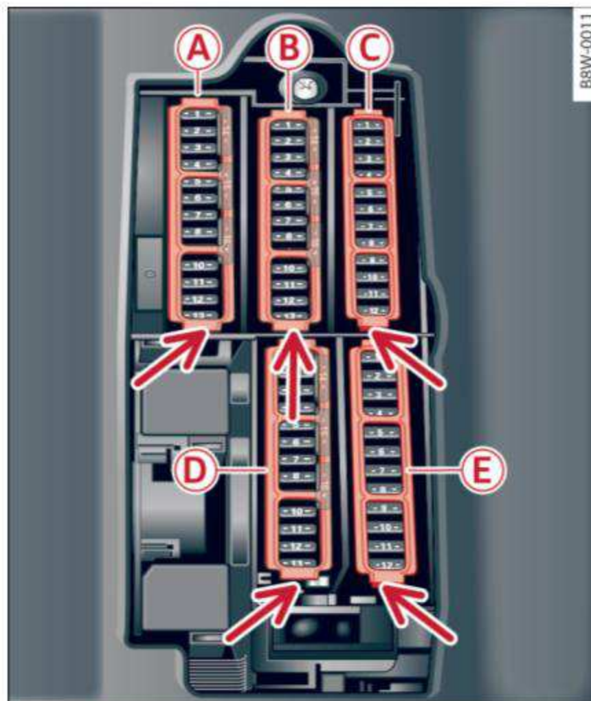
Fig. 282 Driver's footwell (left-hand drive vehicle): fuse panel with plastic clip
