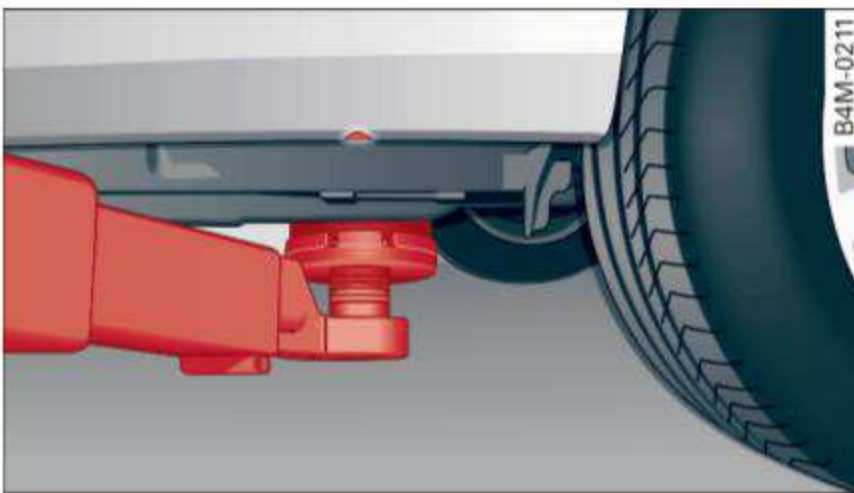
Fig. 292 Rear lifting point
