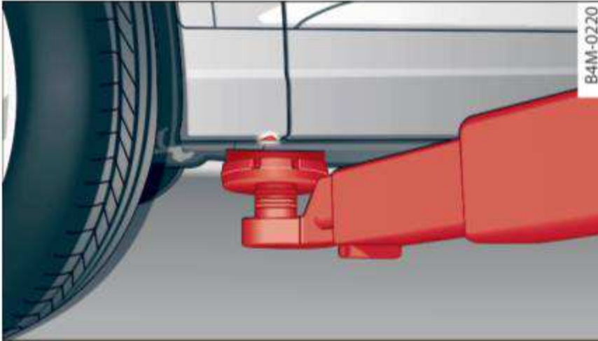
Fig. 291 Front lifting point
