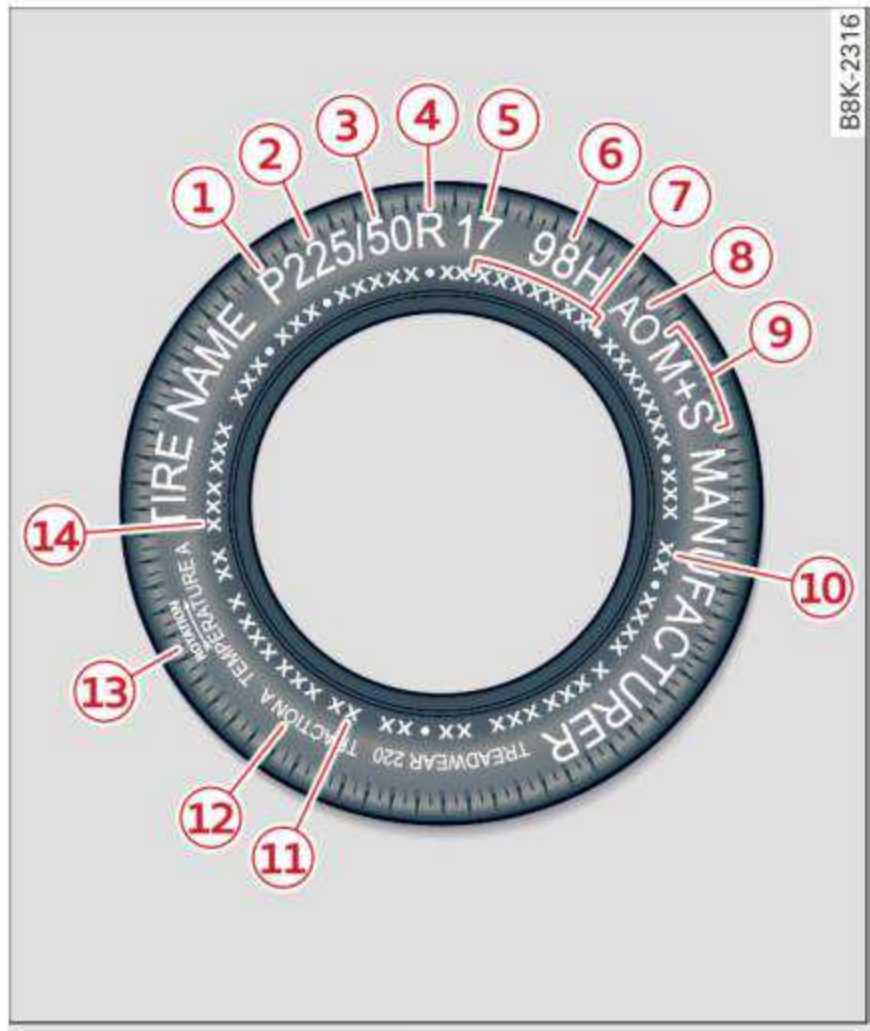
Fig. 266 Tire designations on the sidewall
