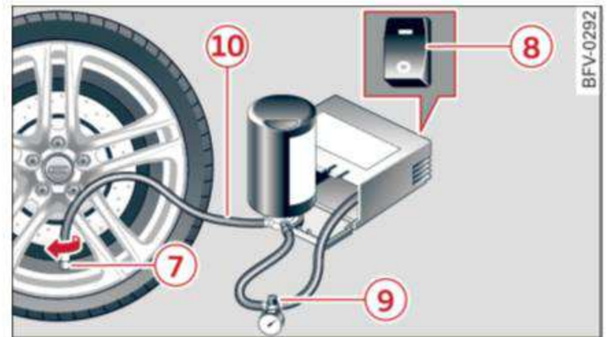
Fig. 273 Tire mobility kit connection
