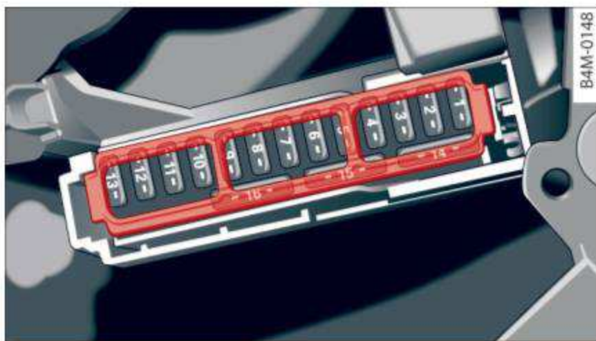
Fig. 284 Driver side cockpit: fuse panel with plastic bracket
