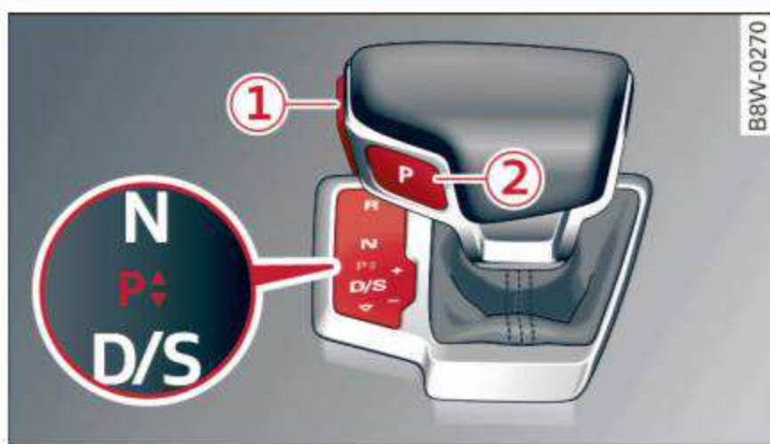
Fig. 90 Center console: selector lever
