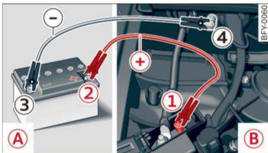
Fig. 287 Jump starting with a battery in another vehicle: (A) - providing current, (B) - drained
