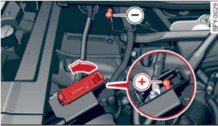
Fig. 264 Engine compartment: connectors for a charger and jump start cables
