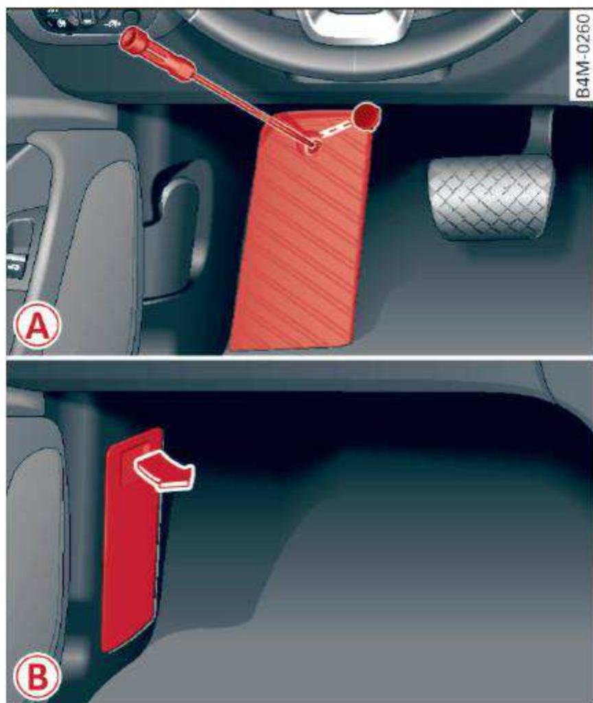
Fig. 280 (A) Driver footwell (left-hand drive vehicle): footrest, (B) Front passenger footwell (right-hand drive vehicle): cover
