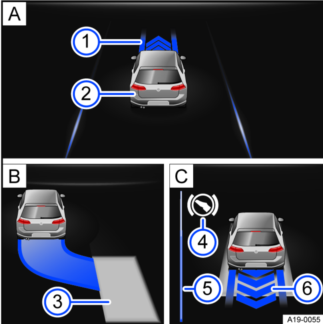
Fig. 117 In the digital instrument cluster display: drive into a parking space parallel to the road (general example).
