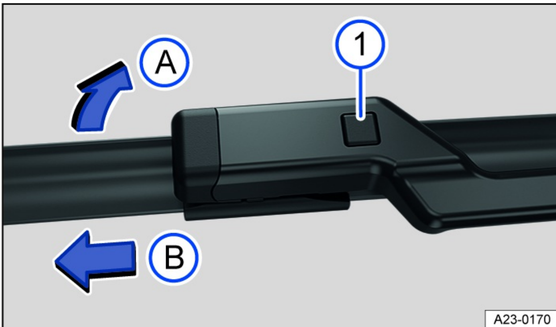
Fig. 150 Changing the windshield wiper blades.
