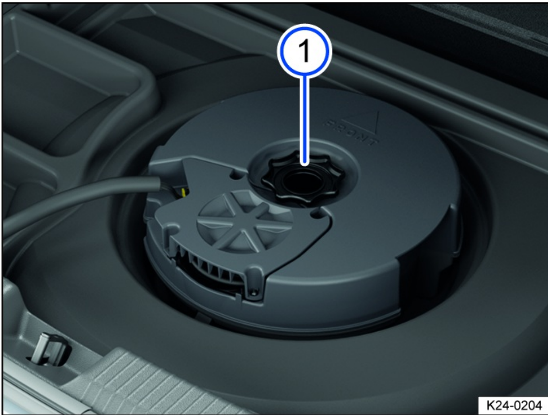
Fig. 183 Under the luggage compartment floor: removing the subwoofer.
