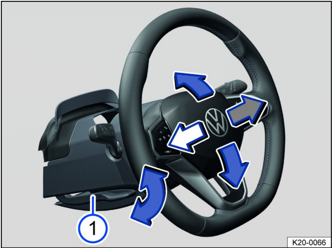
Fig. 55 Under the steering wheel in the steering column trim panel: lever to adjust the steering wheel position manually (general example).
