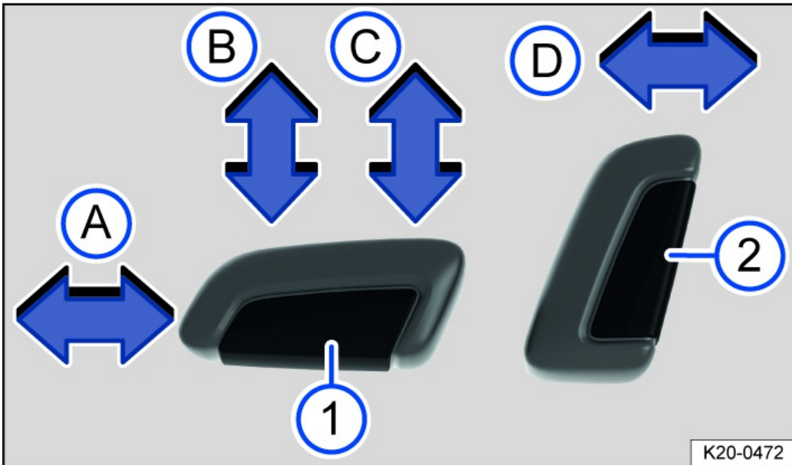
Fig. 58 Switch on the driver seat: Adjusting the front seat forward/back, the height and angle of the seat surface, and the front seat backrest.
