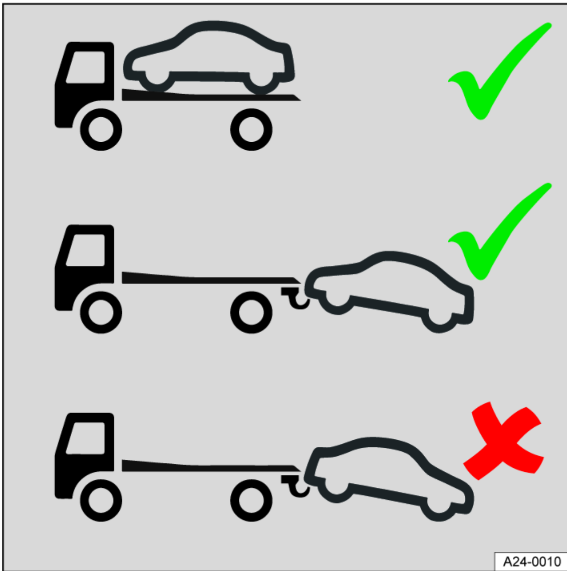
Fig. 160 Transporting the vehicle away with a tow truck.
