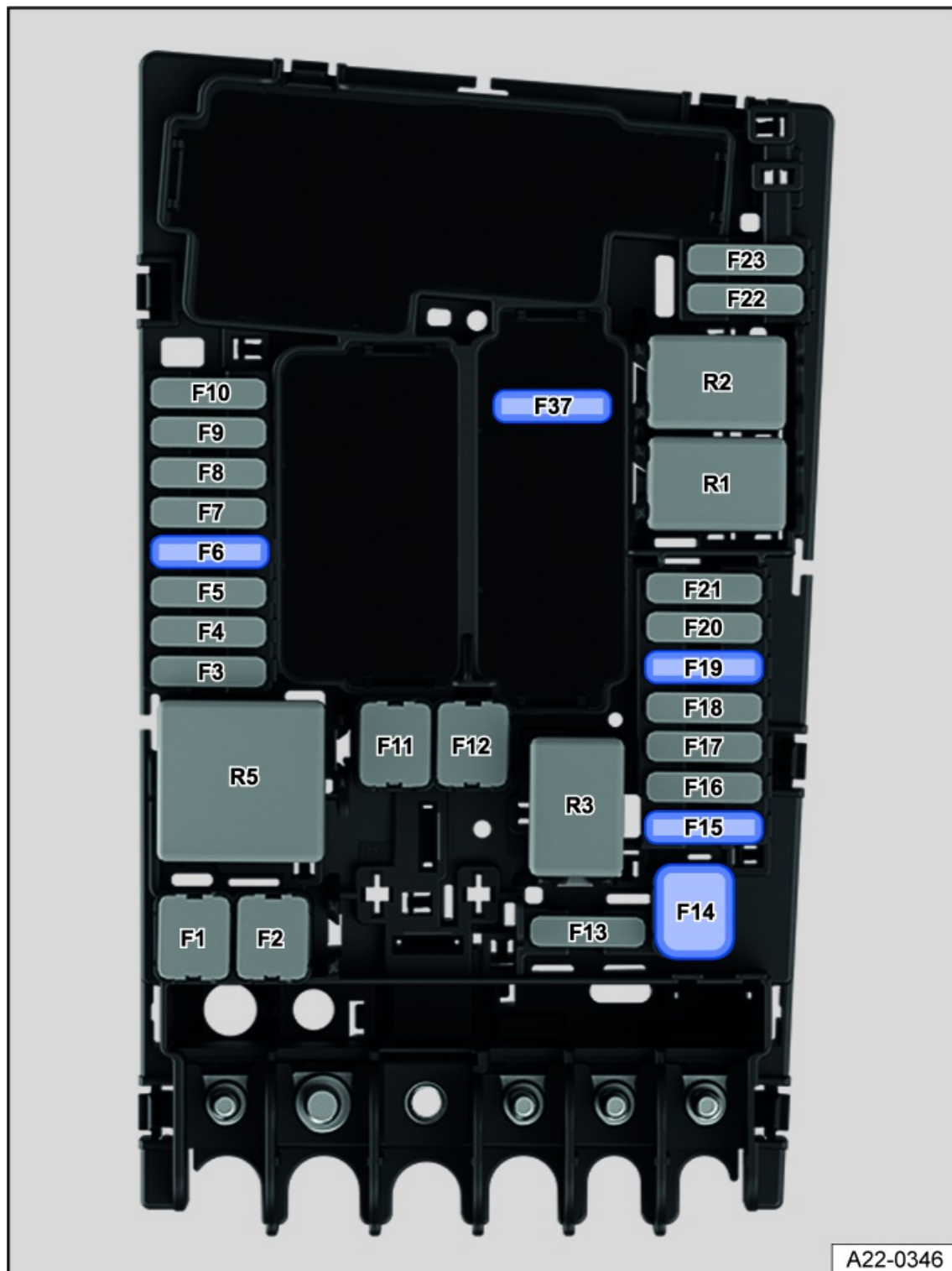
Fig. 153 In the hood space: Fuse locations.
