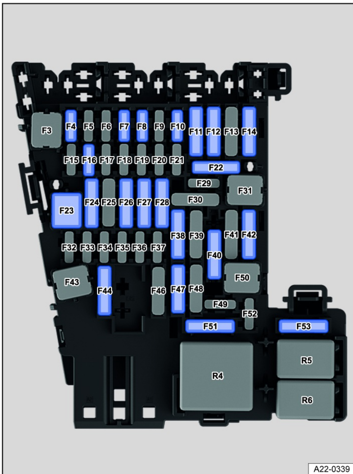
Fig. 155 Fuse assignment in the instrument panel.
