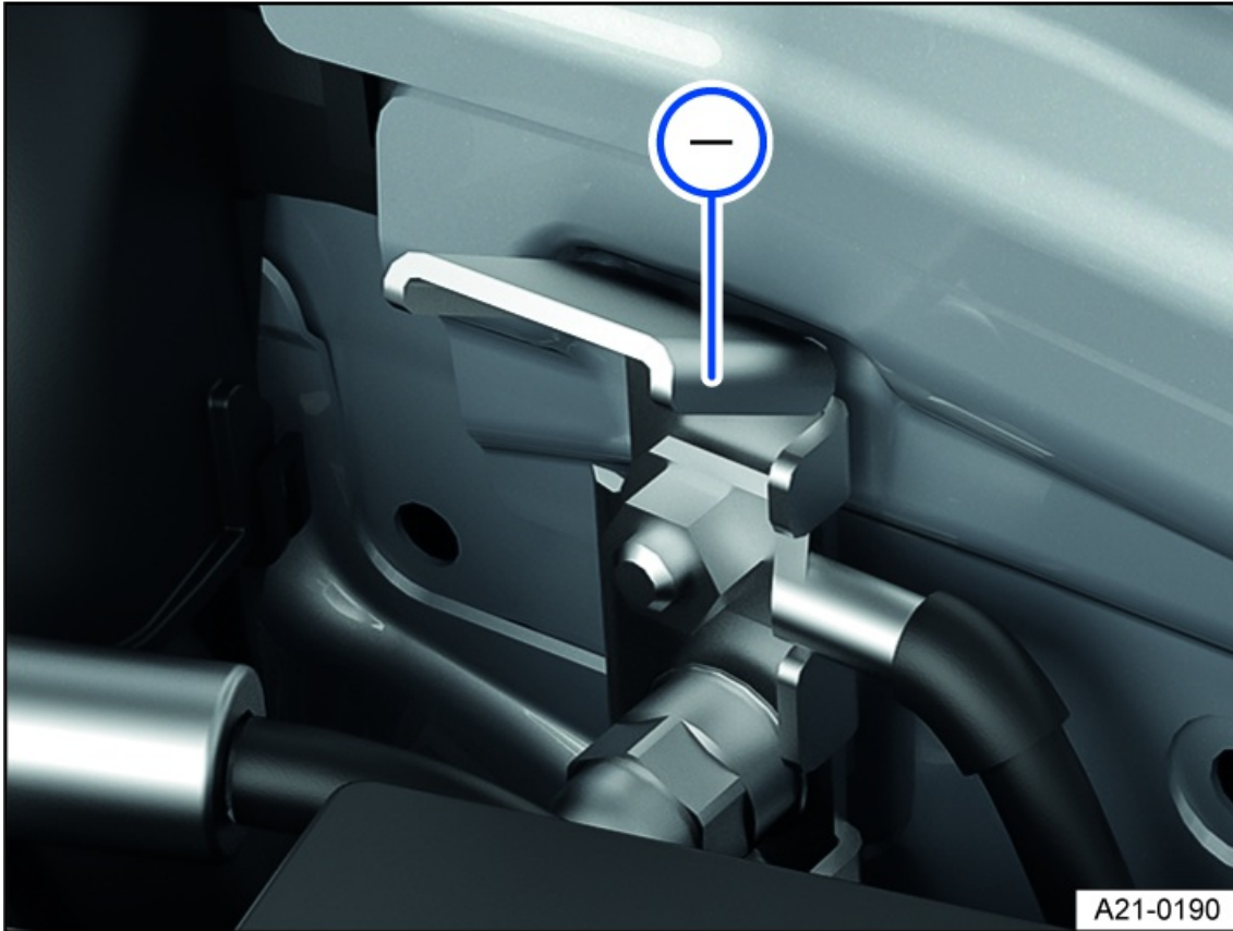
Fig. 158 In the hood space: Negative terminal jump-start point.
