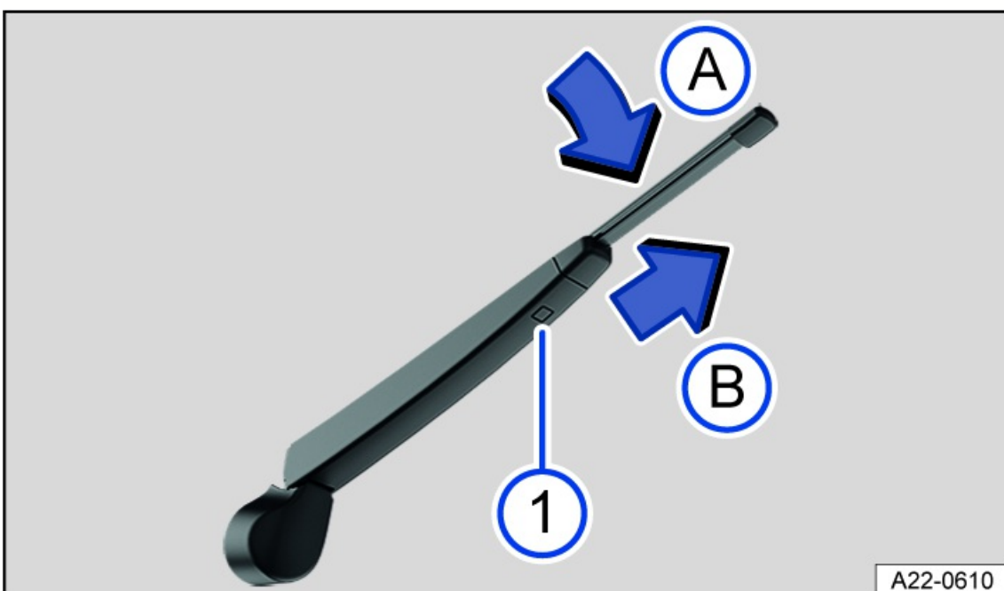
Fig. 151 Changing the rear window wiper blade.
