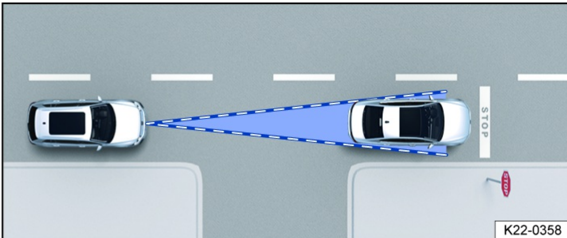
Fig. 104 Stationary vehicle.
