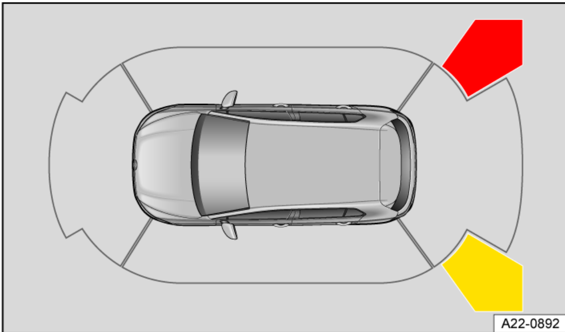
Fig. 122 Infotainment system: Rear Traffic Alert display (depending on the vehicle equipment).
