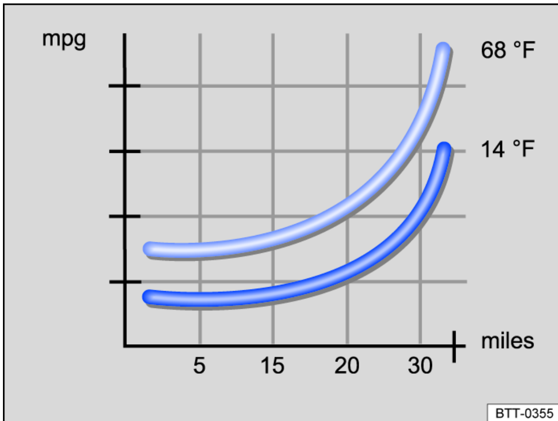
Fig. 100 Fuel consumption in mpg at two different ambient temperatures.
