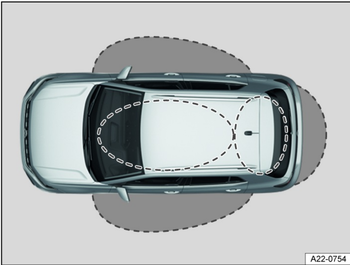
Fig. 42 Keyless Access: Sensor ranges (general example).
