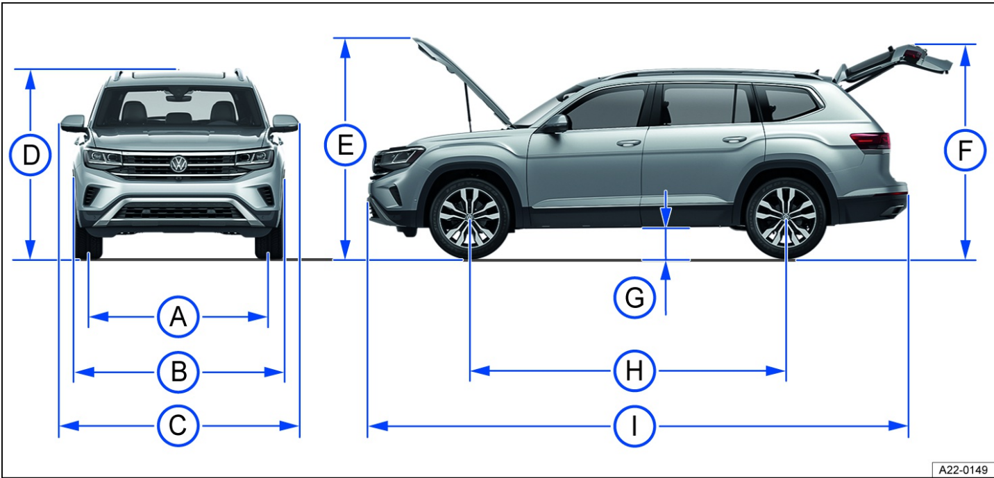
Fig. 222 Vehicle dimensions.
