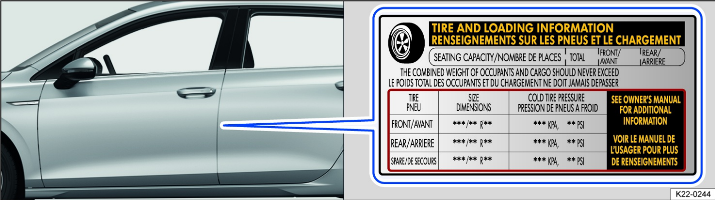
Fig. 197 On the driver door pillar: Tire inflation pressure label.
