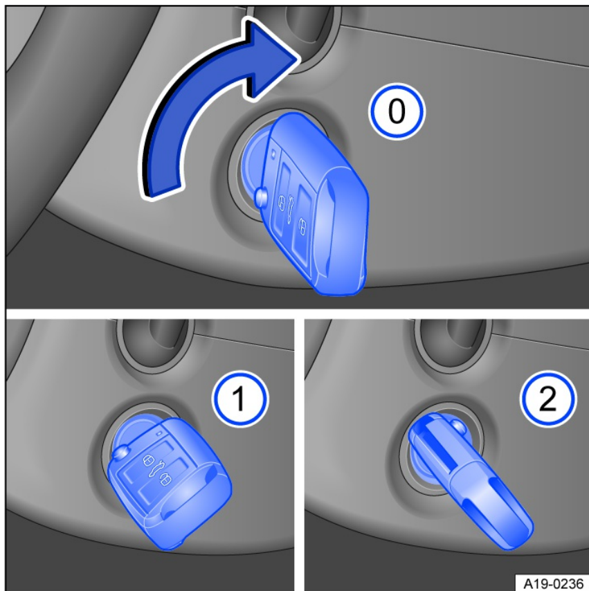
Fig. 110 Next to the steering wheel on the right side: positions of the vehicle key in the ignition lock.
