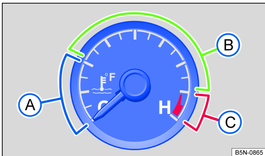
Fig. 23 Engine coolant temperature gauge in the analog instrument cluster.
