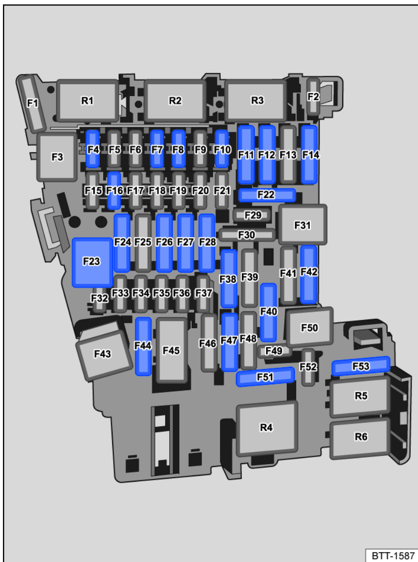
Fig. 179 Fuse assignment in the instrument panel.
