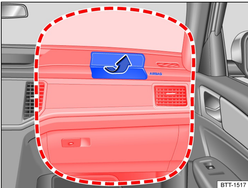
Fig. 34 Installation location and deployment zone of the front passenger's front airbag.
