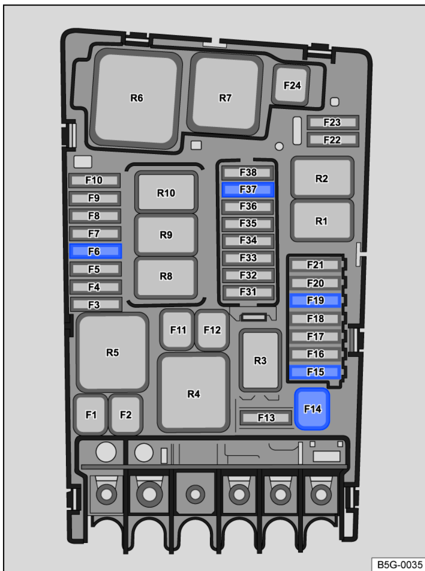
Fig. 177 Fuse locations in the engine compartment.
