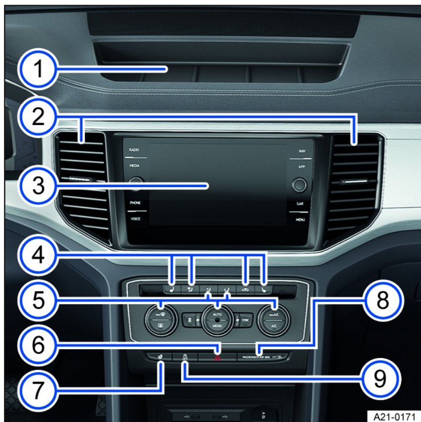
Fig. 6 Overview of the upper section of the center console.
