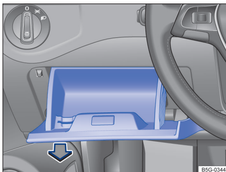
Fig. 156 On the driver side in the instrument panel: Removing the storage compartment to access fuses.
