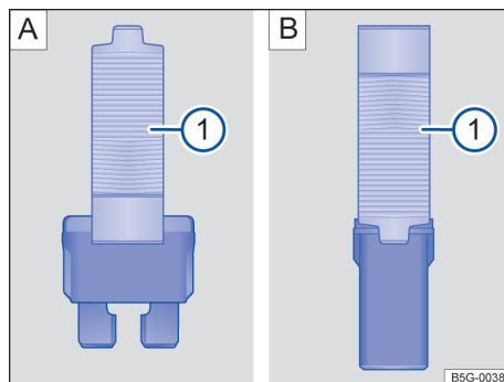
Fig. 159 Removing or installing a blade fuse with the plastic tweezers: A : Blade fuse. B : JCASE® fuse.
