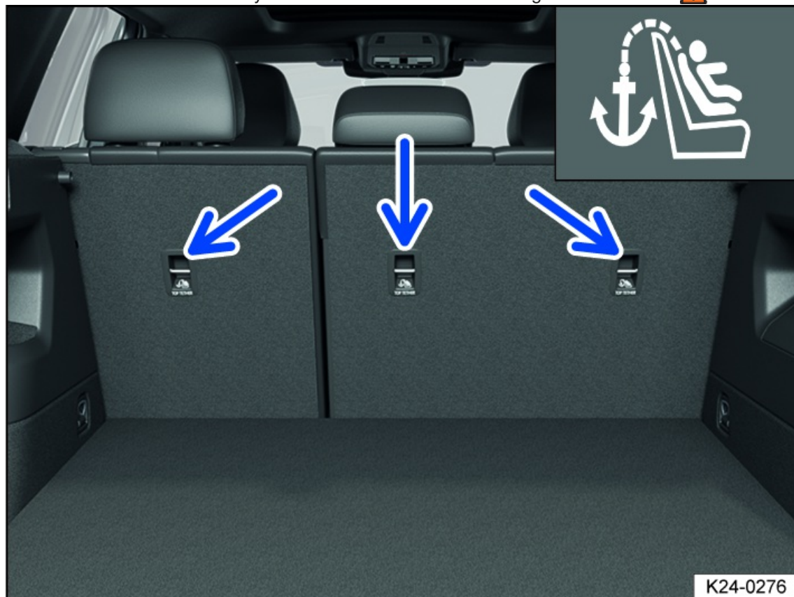
Fig. 29 On the back of the rear seats of the second-row seats: top tether anchorages for the top tether safety belt.
