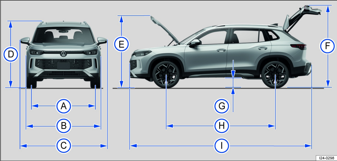
Fig. 187 Vehicle dimensions.
