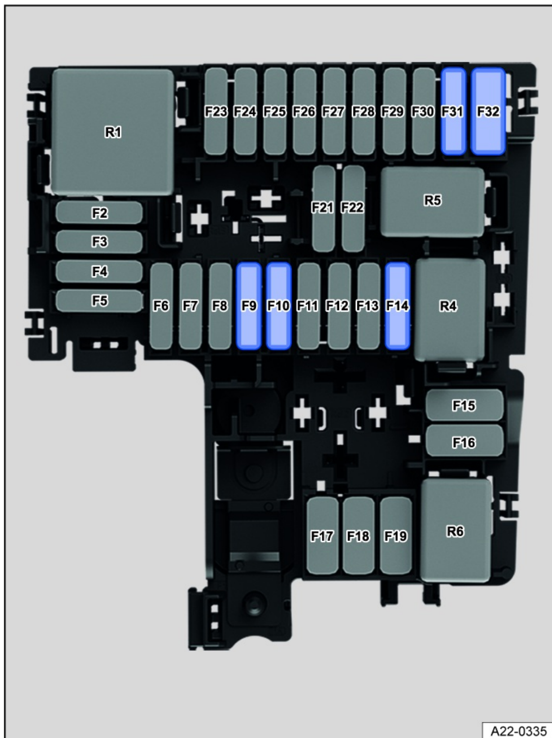
Fig. 144 In the hood space: Fuse locations.
