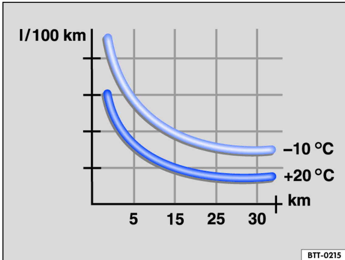
Fig. 95 Fuel consumption in l/100 km (mpg) for two different environmental temperatures.
