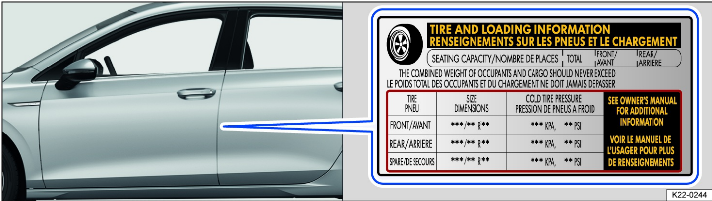
Fig. 167 On the driver door pillar: Tire inflation pressure label.
