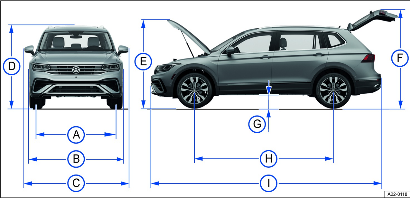
Fig. 235 Vehicle dimensions.
