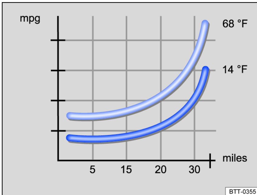
Fig. 126 Fuel consumption in mpg at two different ambient temperatures.
