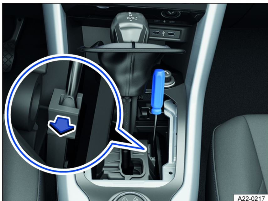
Fig. 124 In the center console: manually release the Automatic Shift Lock (ASL) (variant 2).
