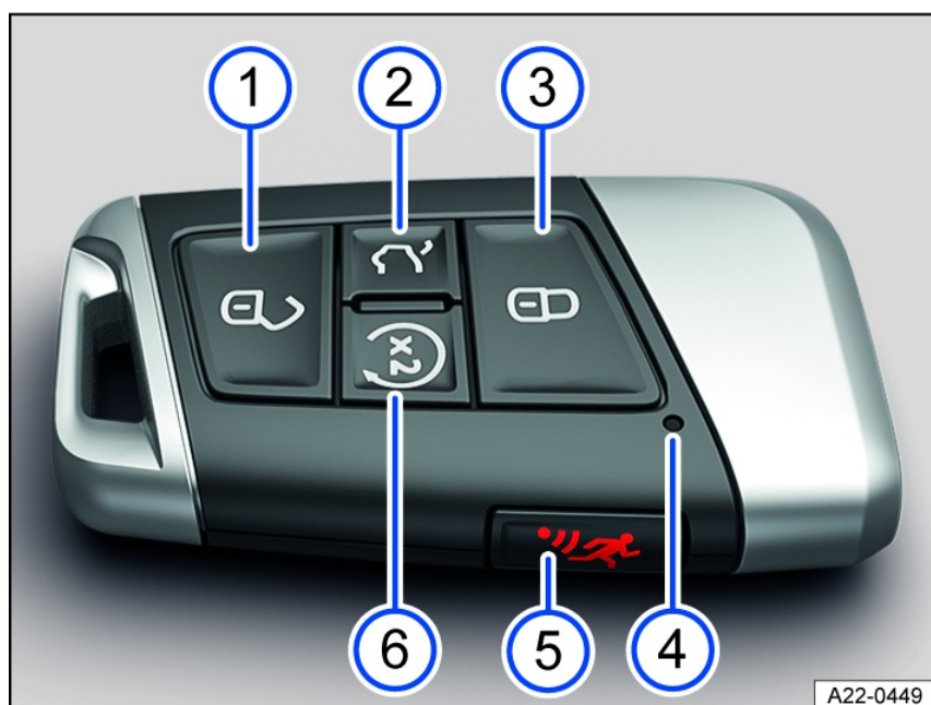
Fig. 52 Vehicle key with remote start relay function.
