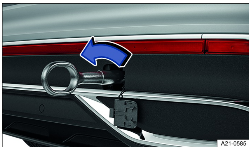
Fig. 199 In the right rear bumper: Screw in towing eye, variant 1.
