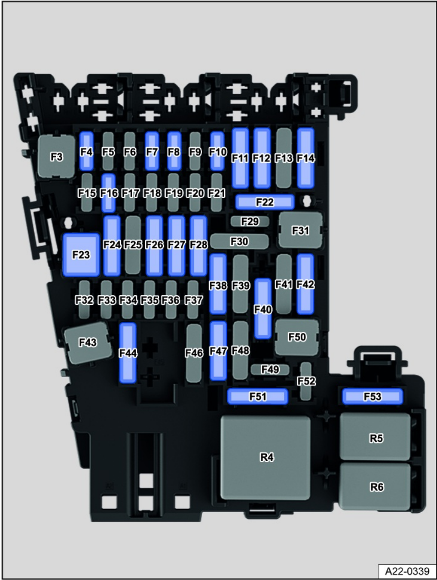
Fig. 190 Fuse assignment in the instrument panel.
