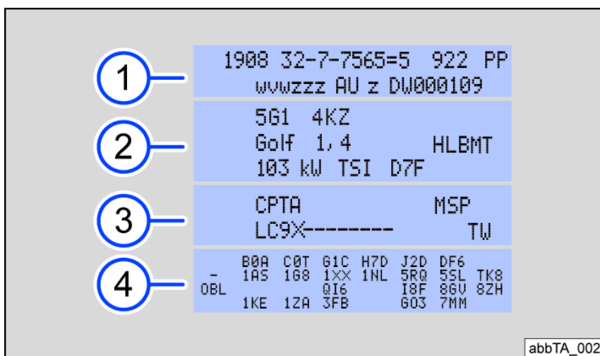
Fig. 225 General example: vehicle data label.
