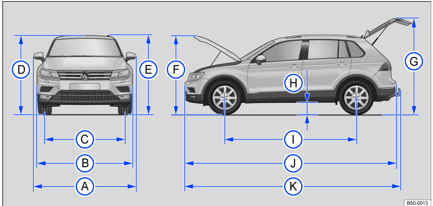
Fig. 226 Vehicle dimensions.
