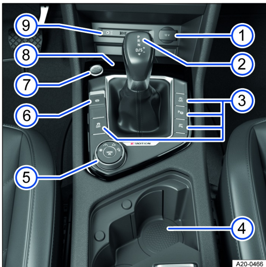
Fig. 8 Overview of the lower section of the center console.
