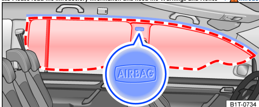
Fig. 38 On the left side of the vehicle (5-seater): installation location and deployment zone of the Side Curtain Protection® airbag.
