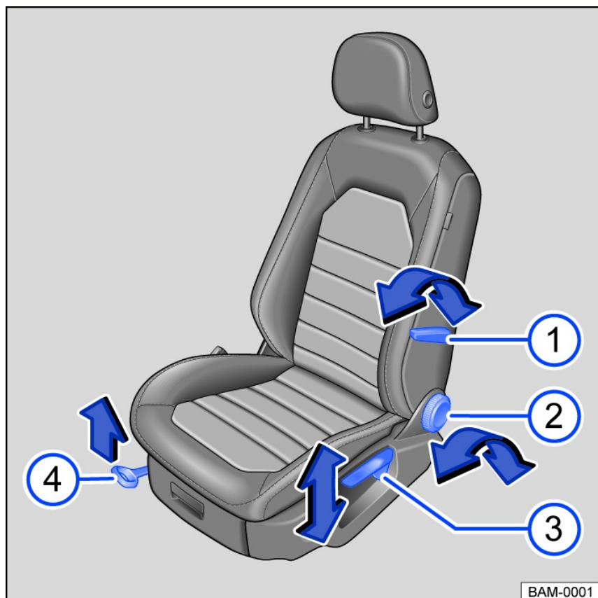
Fig. 71 On the left front seat: Controls (Version 1).
