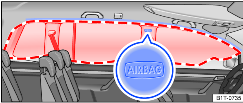
Fig. 39 On the left side of the vehicle (7-seater): installation location and deployment zone of the Side Curtain Protection® airbag.
