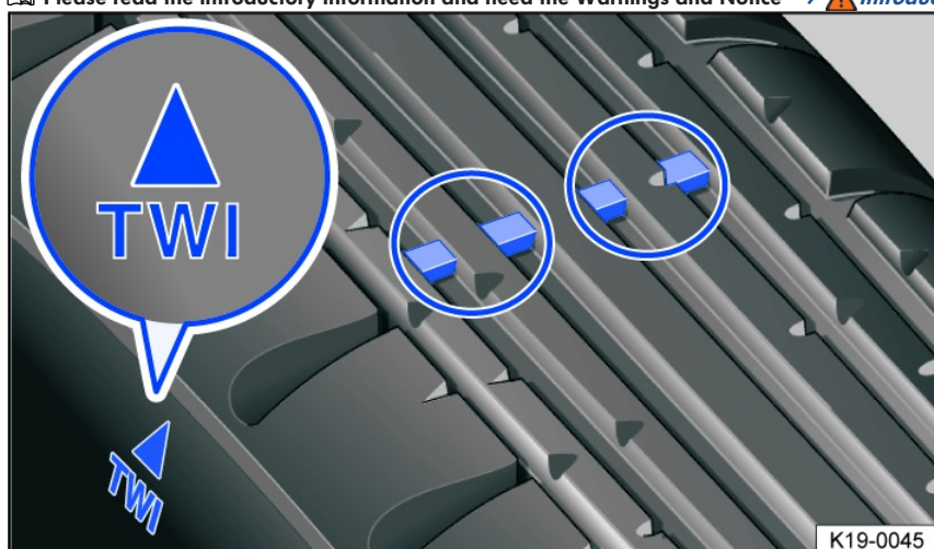
Fig. 206 Tire tread: tread wear indicator.
