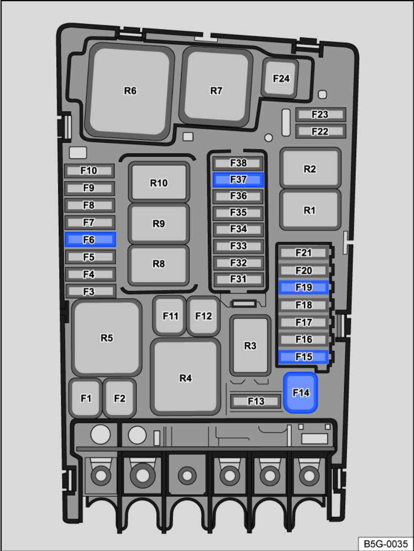
Fig. 179 Fuse locations in the engine compartment.
