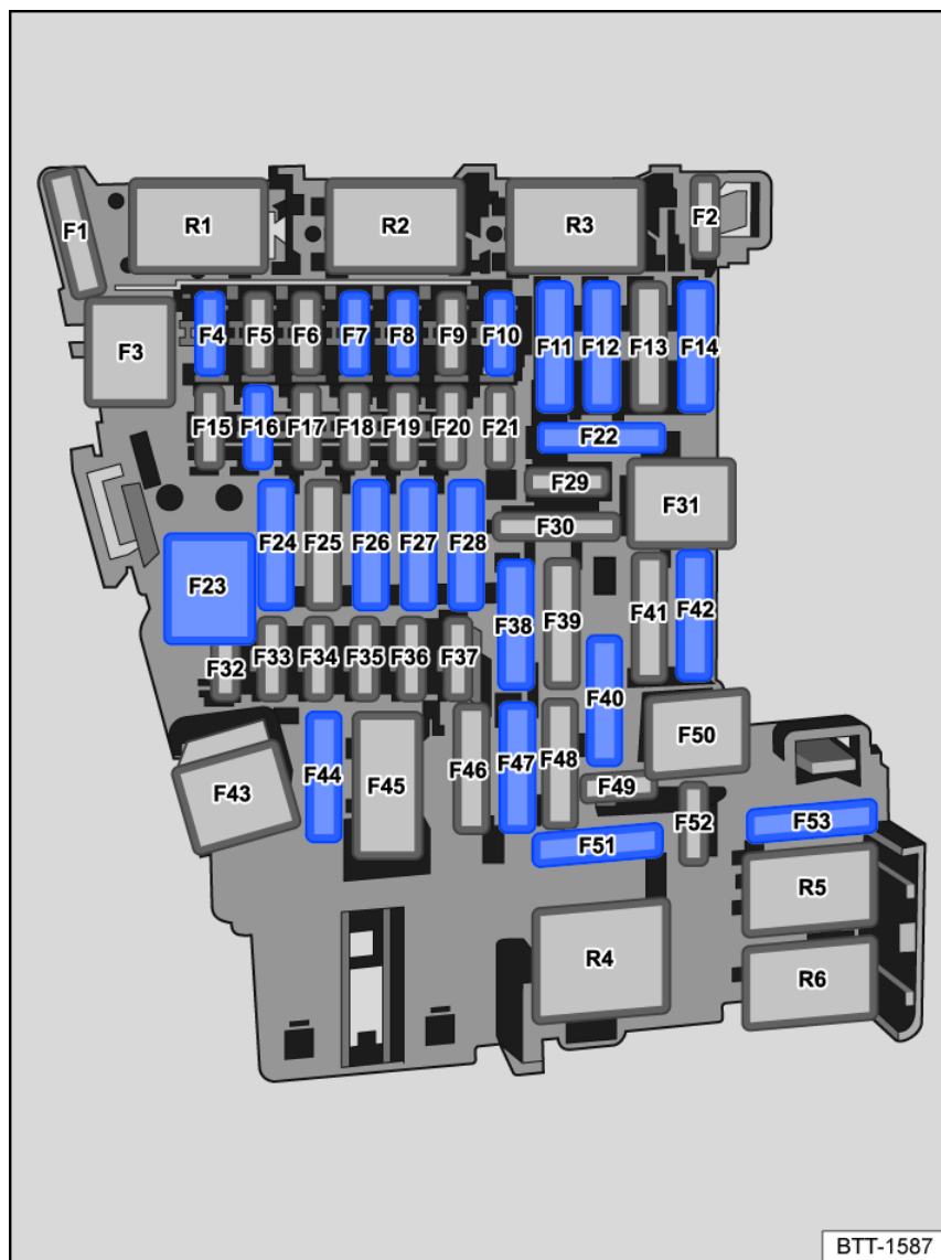
Fig. 182 Fuse assignment in the instrument panel.
