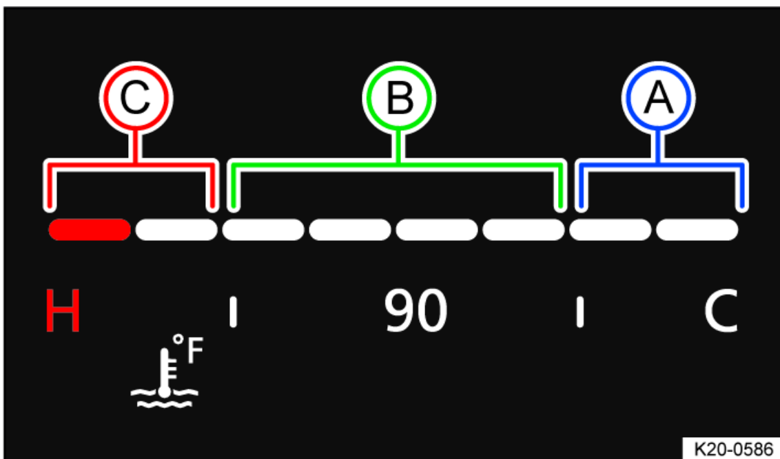
Fig. 18 In the Volkswagen Digital Cockpit Basic: coolant temperature gauge (general example).
