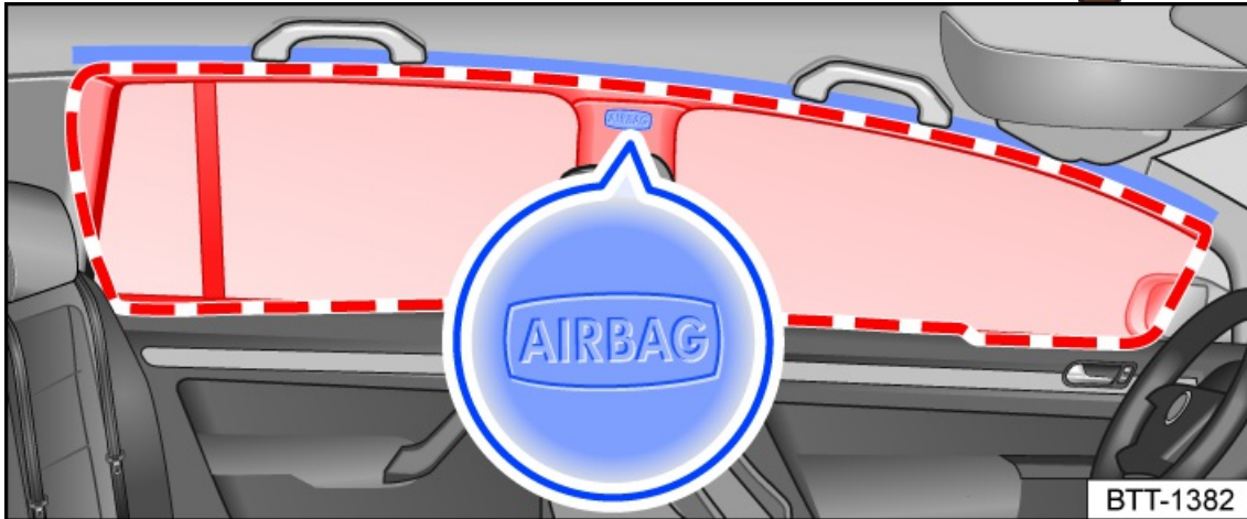
Fig. 34 On the left side of the vehicle: installation location and deployment zone of the Side Curtain Protection®.
