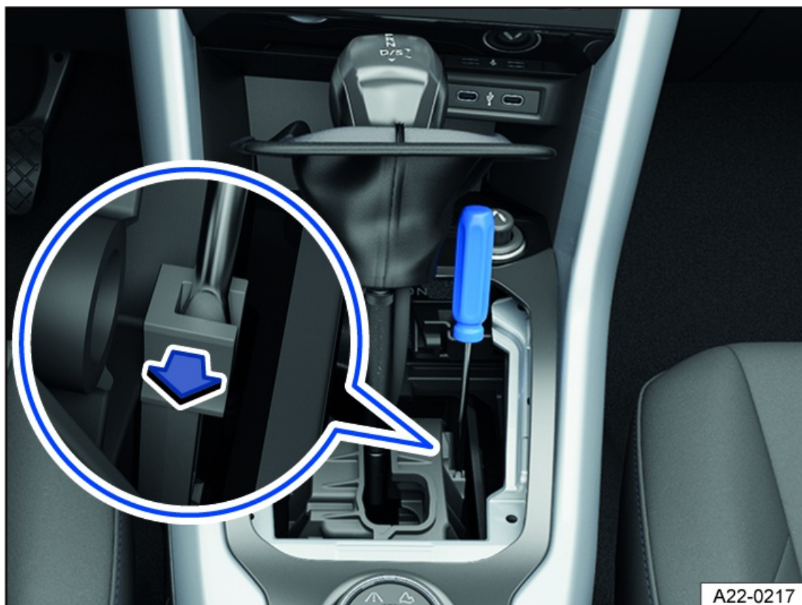
Fig. 103 In the center console: manually release the Automatic Shift Lock (ASL) (variant 2).
