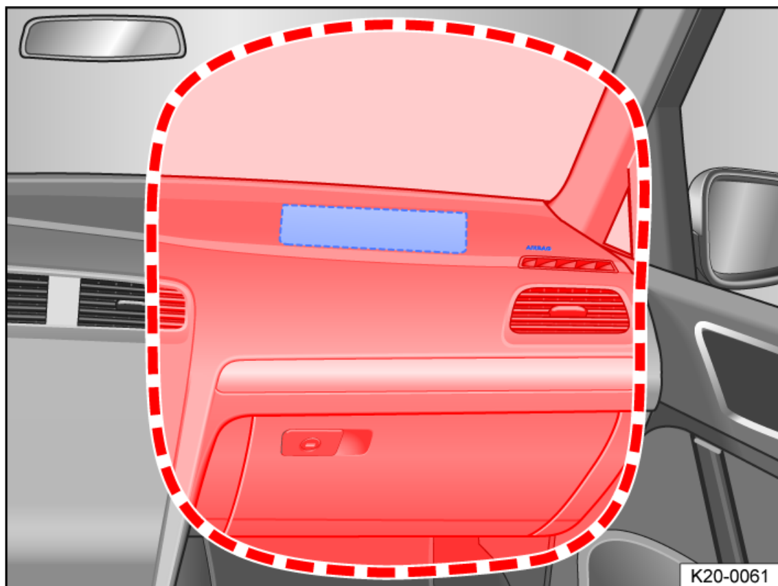
Fig. 31 On the passenger's side: Installation location and deployment zone of the front passenger's front airbag.
