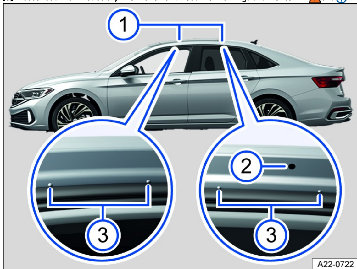
Fig. 135 Mounting points for base supports.
