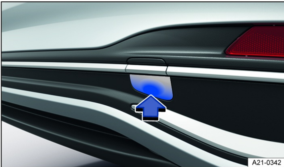
Fig. 155 In the right rear bumper: Remove cover.
