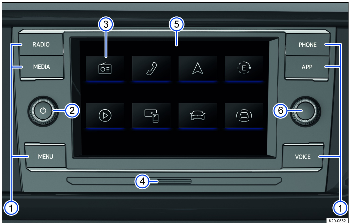
Fig. 133 Overview of the Infotainment system in the 6.5" version.
