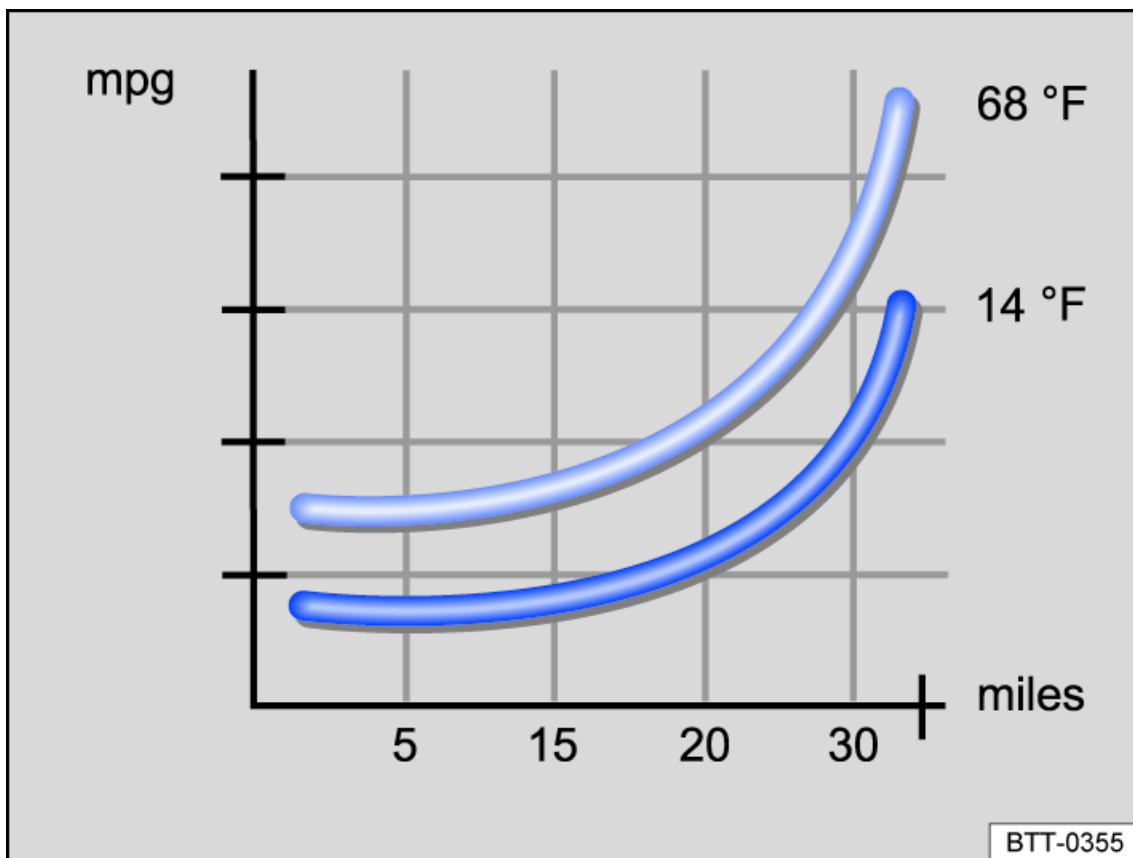
Fig. 107 Fuel consumption in mpg at two different ambient temperatures.
