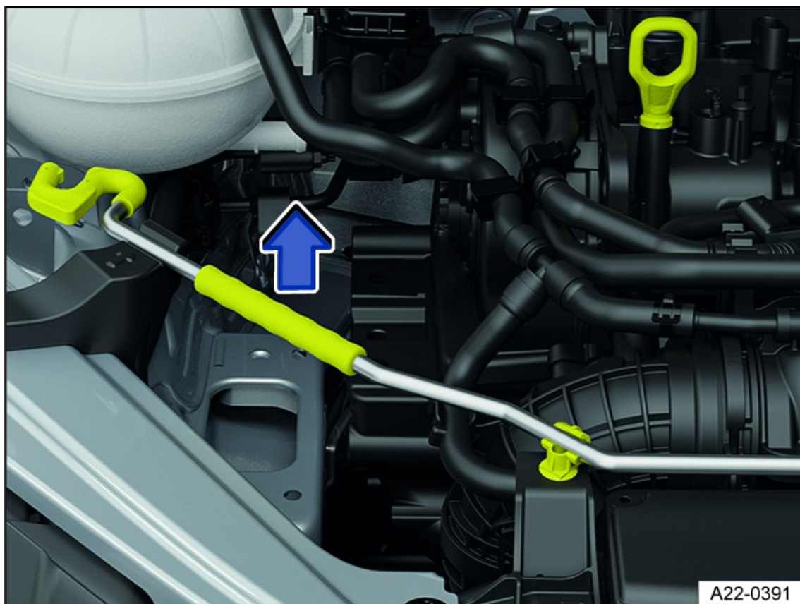
Fig. 161 In the engine compartment: Hood support in the bracket.
