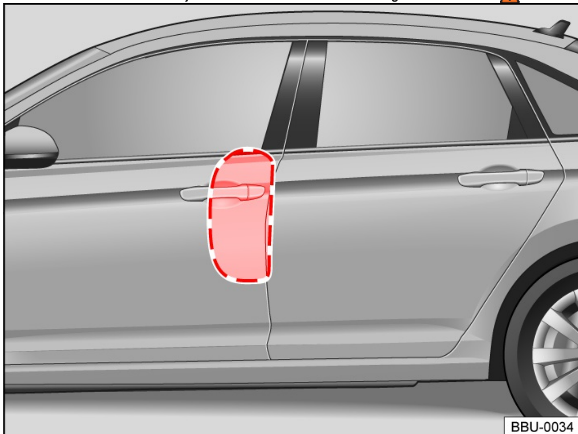
Fig. 32 In the vehicle interior on the left side of the vehicle: deployment zones of the side airbag.
