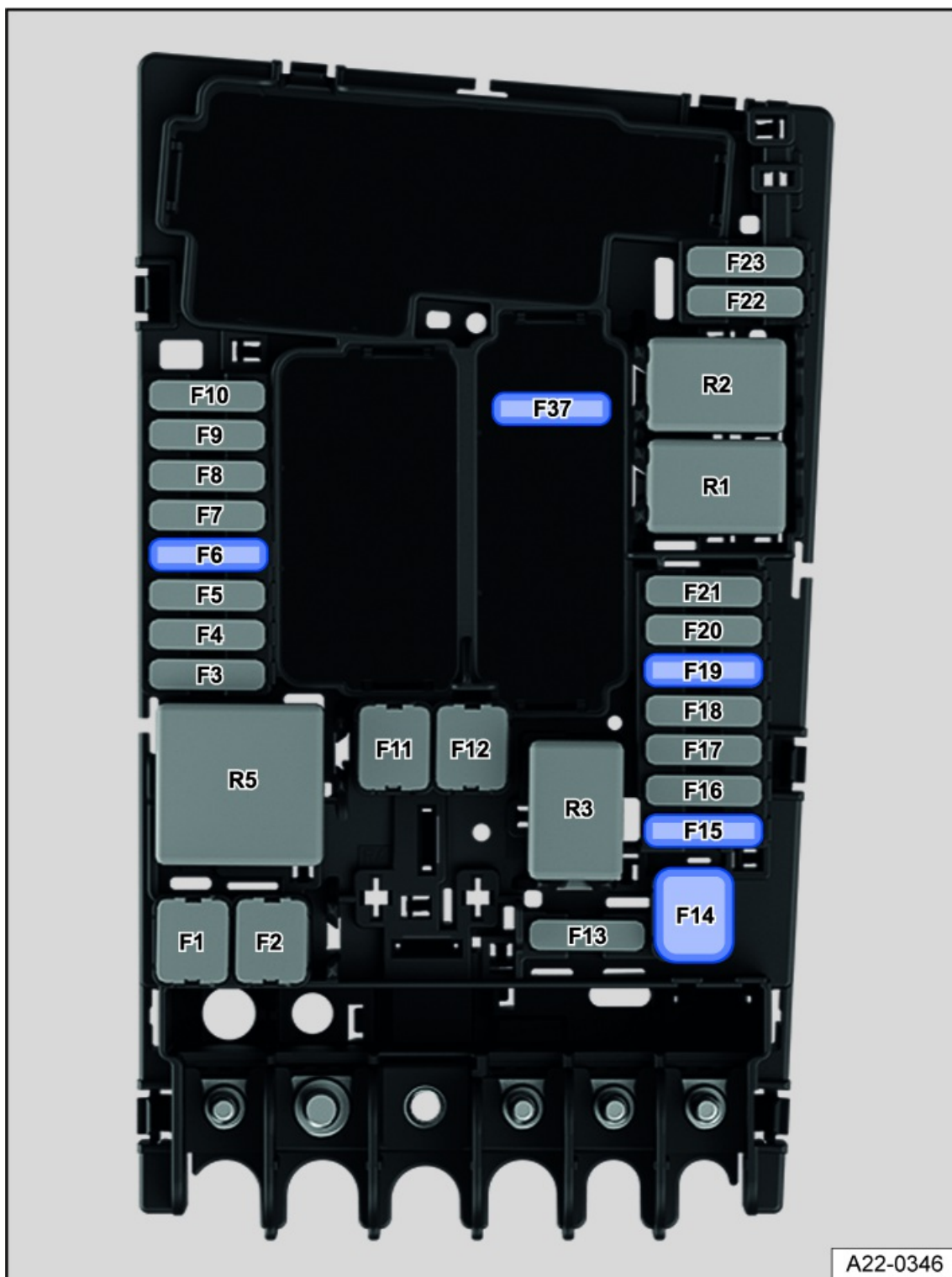
Fig. 144 Fuse locations in the engine compartment.
