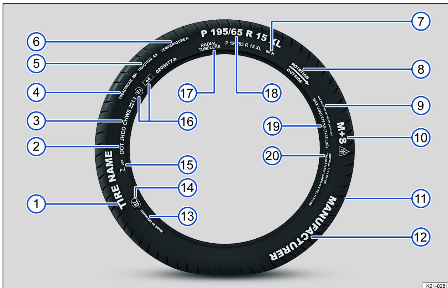
Fig. 192 International tire labeling.
