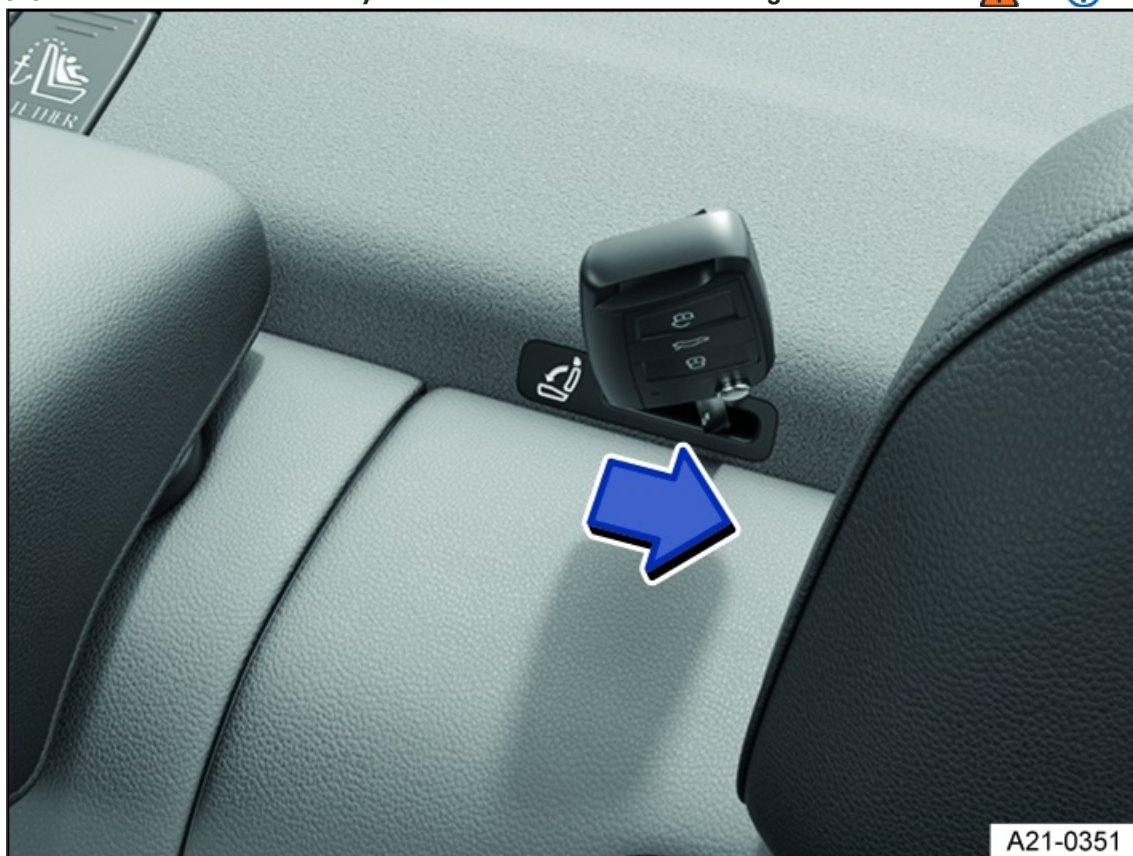
Fig. 60 Behind the rear seat backrest: mechanically unlocking the rear seat backrest using the emergency release.
