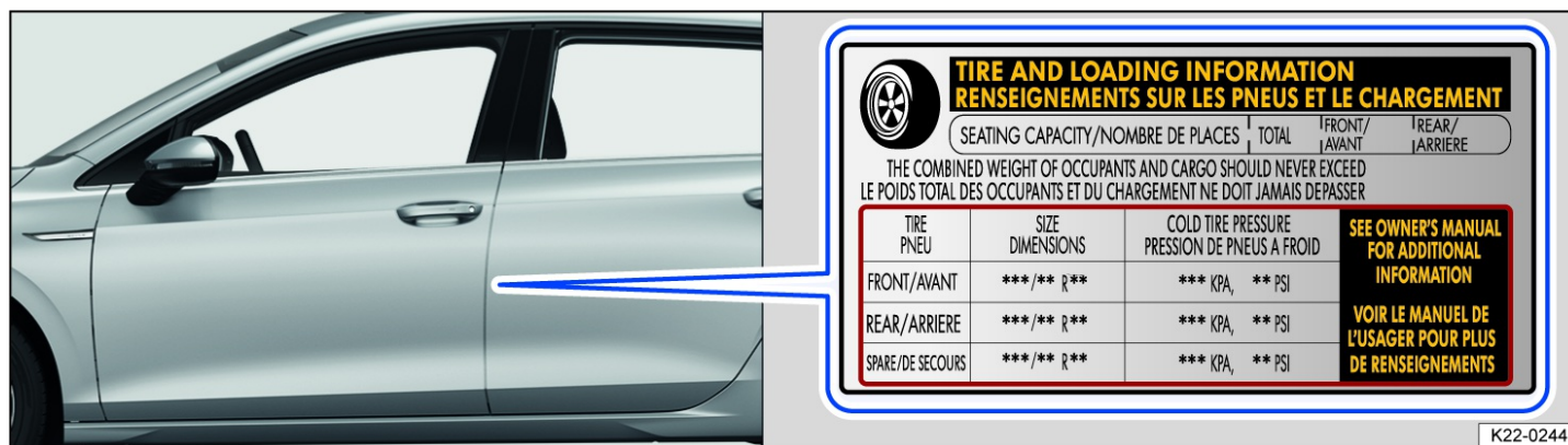
Fig. 172 On the driver door pillar: Tire inflation pressure label.
