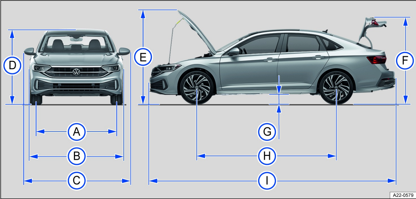
Fig. 201 Vehicle dimensions.
