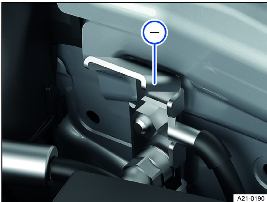
Fig. 149 In the engine compartment: Negative terminal jump-start point.
