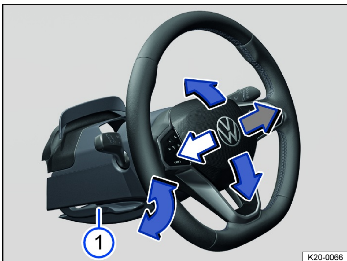
Fig. 64 Under the steering wheel in the steering column trim panel: lever to adjust the steering wheel position manually (general example).
