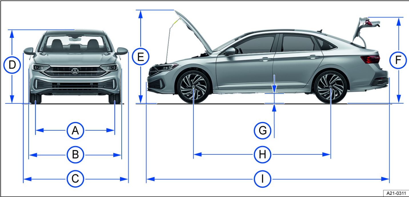
Fig. 196 Vehicle dimensions.
