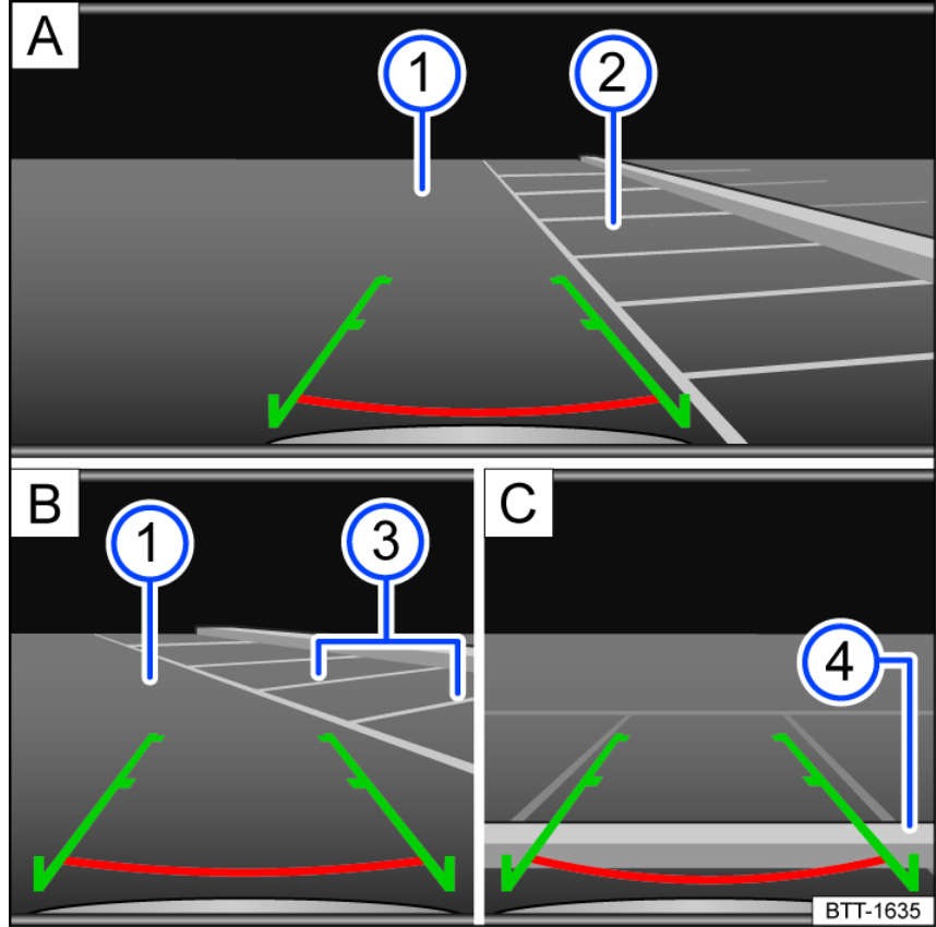
Fig. 122 Infotainment system: Parking with the Rear View Camera system.
