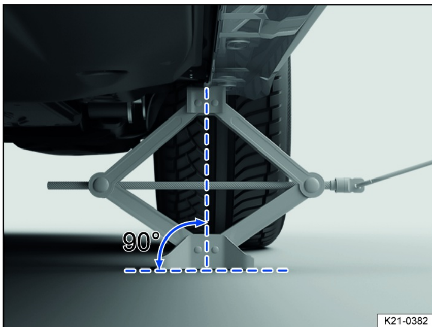
Fig. 179 Jack positioned on the left side of the vehicle at the rear (variant 1).
