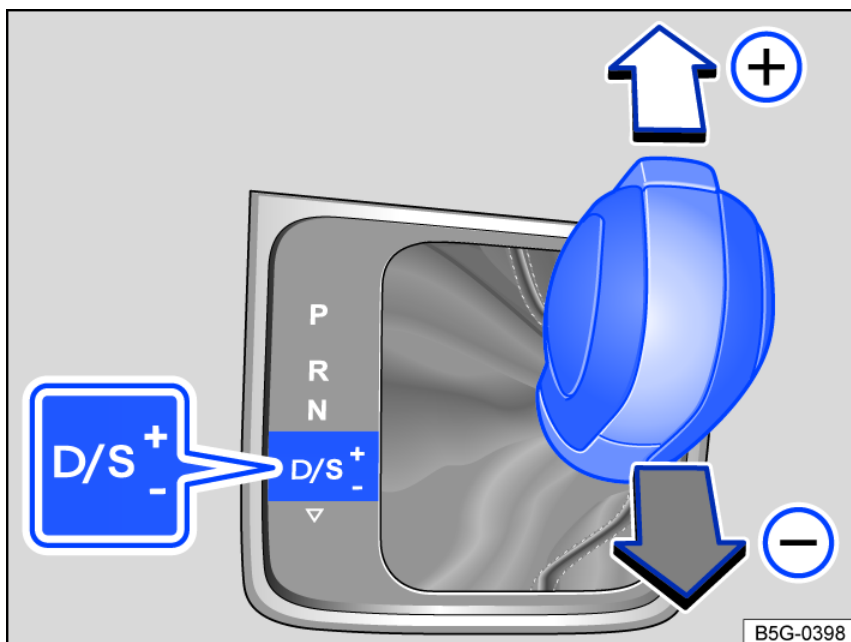
Fig. 99 Selector lever in Tiptronic position.
