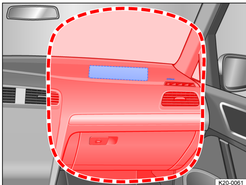
Fig. 31 Installation location and deployment zone of the front passenger's front airbag.
