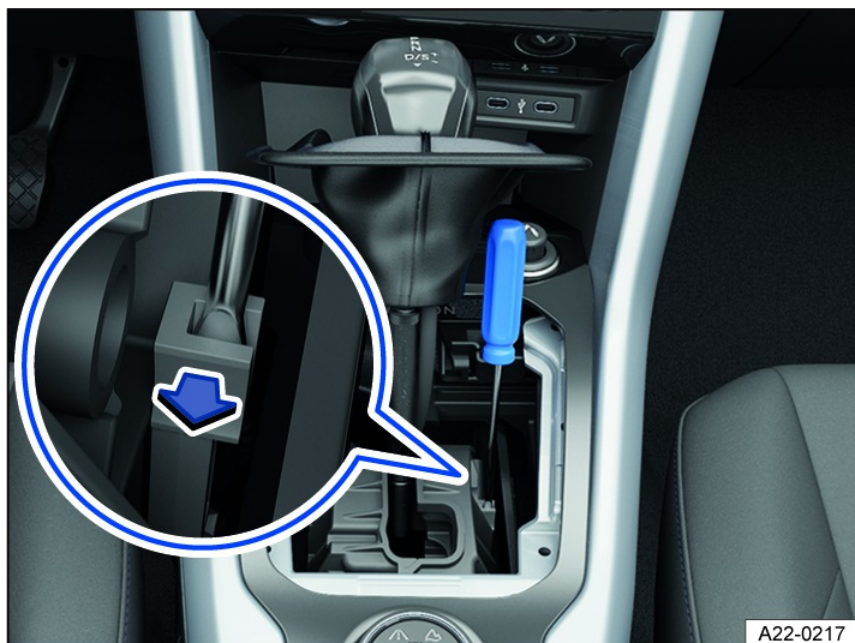
Fig. 102 In the center console: manually release the Automatic Shift Lock (ASL) (variant 2).
