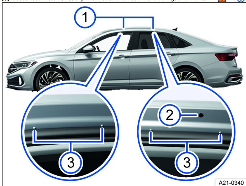
Fig. 132 Mounting points for base supports.
