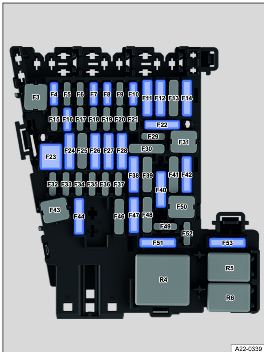
Fig. 143 Fuse assignment in the instrument panel.
