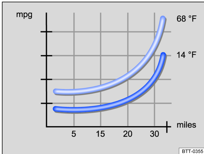
Fig. 104 Fuel consumption in mpg at two different ambient temperatures.
