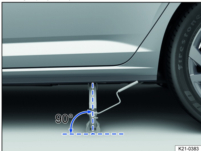
Fig. 178 Correct jack setup (variant 1).
