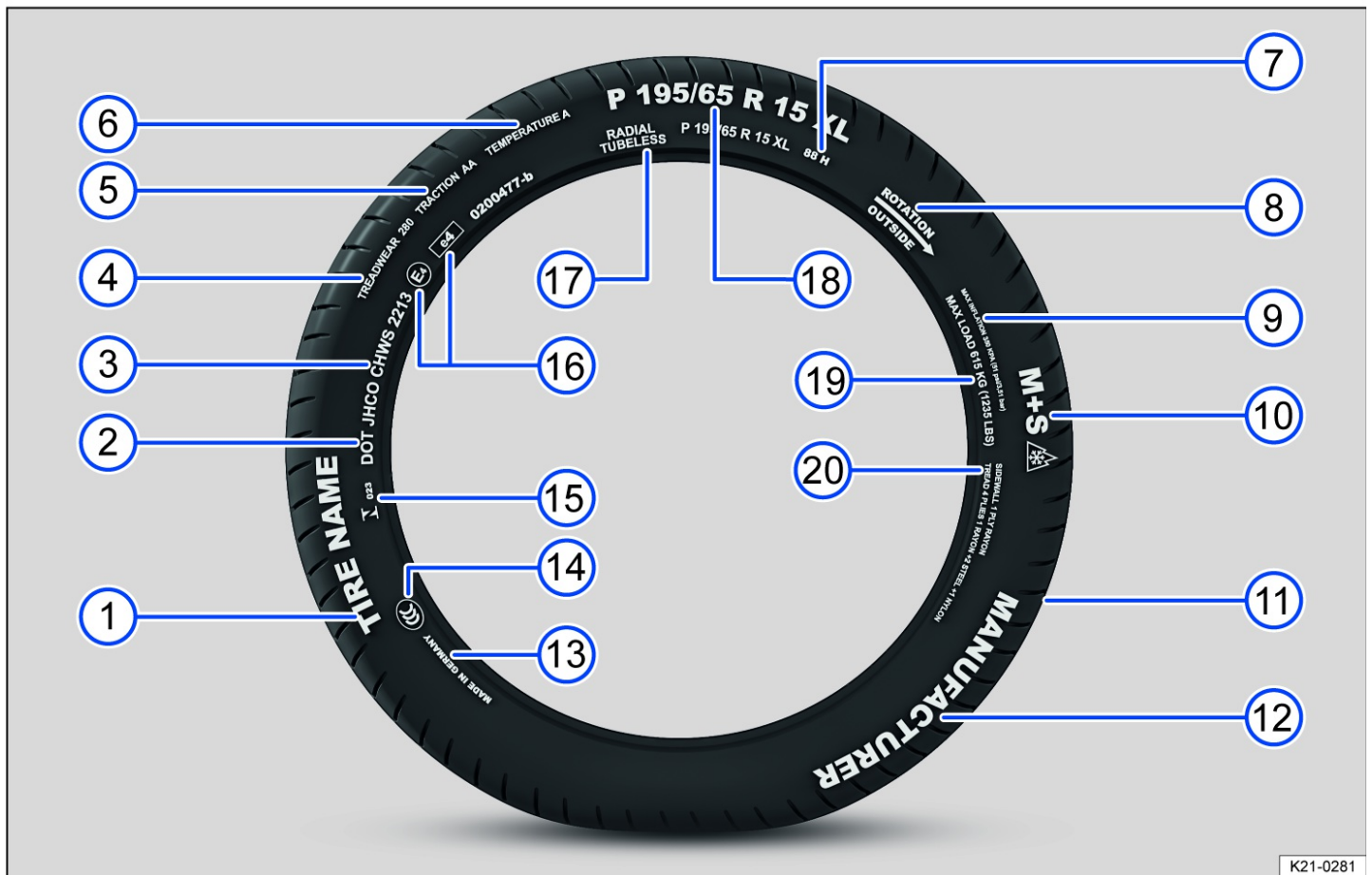
Fig. 184 International tire labeling.
