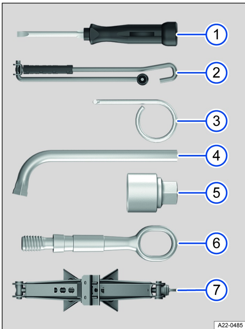
Fig. 135 Vehicle tool kit components (general example).
