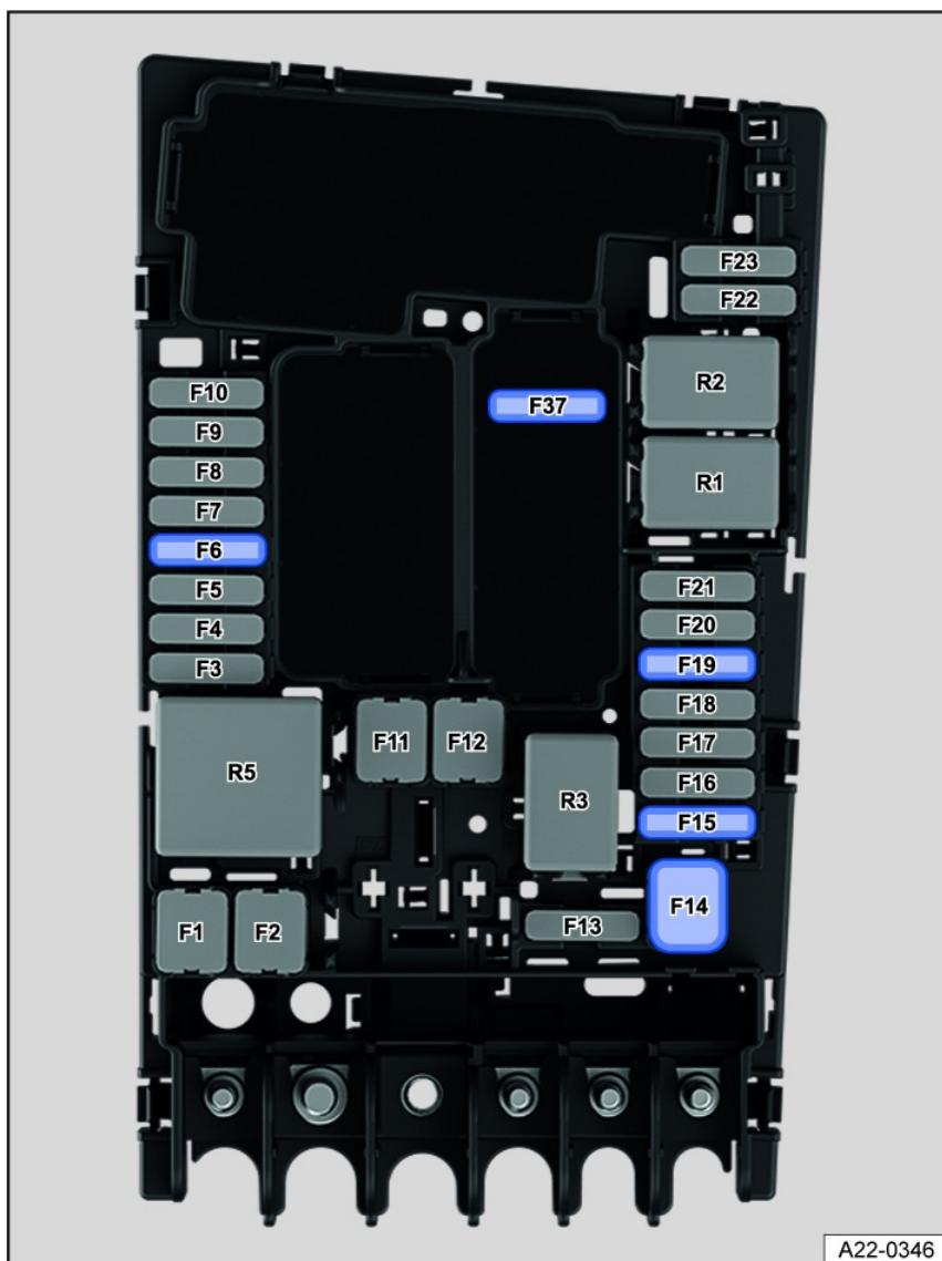
Fig. 141 Fuse locations in the engine compartment.
