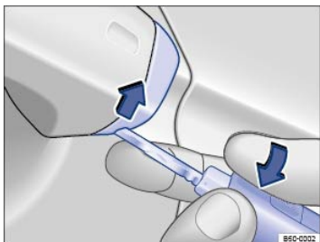
Fig. 61 Driver door handle: Removing the lock cylinder cover.
