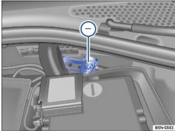
Fig. 151 In the engine compartment: Negative jump-start terminal ⊖.
