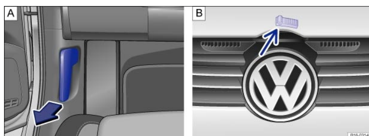
Fig. 157 : In the footwell on the driver side: Inside engine hood release lever. : Above the radiator grille: Outside engine hood release.
