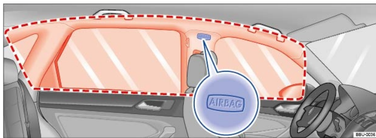
Fig. 39 On the left vehicle side: Installation location and deployment zone of the Side Curtain Protection airbag.
