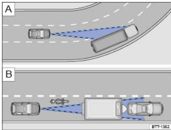
Fig. 119 Driving in a curve. Motorcycle traveling ahead outside of the sensor range.
