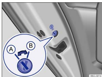
Fig. 64 In the rear driver side door: Child safety lock (A) deactivated, (B) activated.
