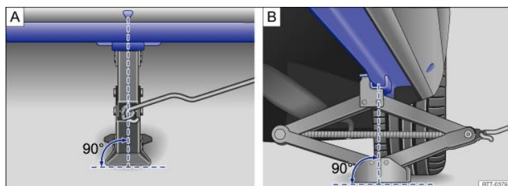
Fig. 179 Jack in position at the left rear lift point.
