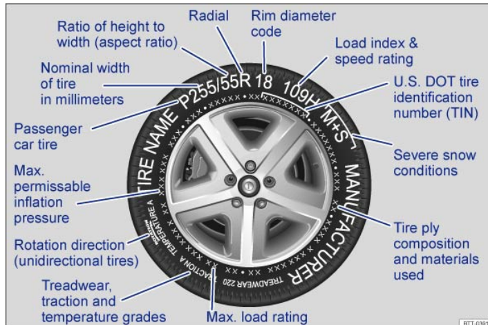
Fig. 172 International tire labeling.
