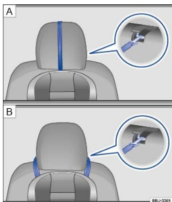
Fig. 47 Examples of mounted top tether straps.
