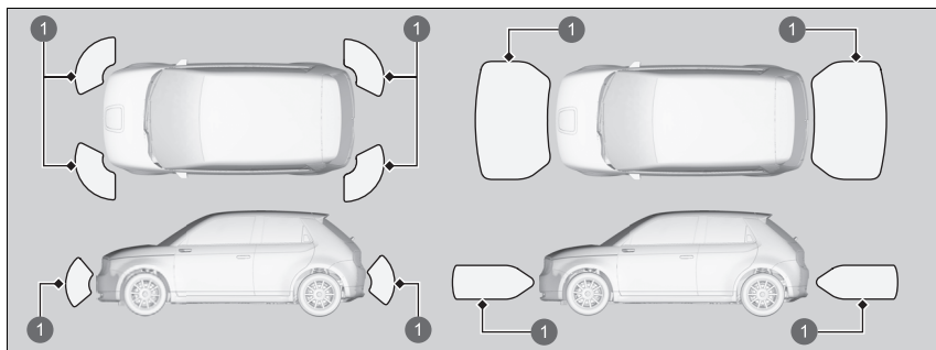
1 Sensor Range
